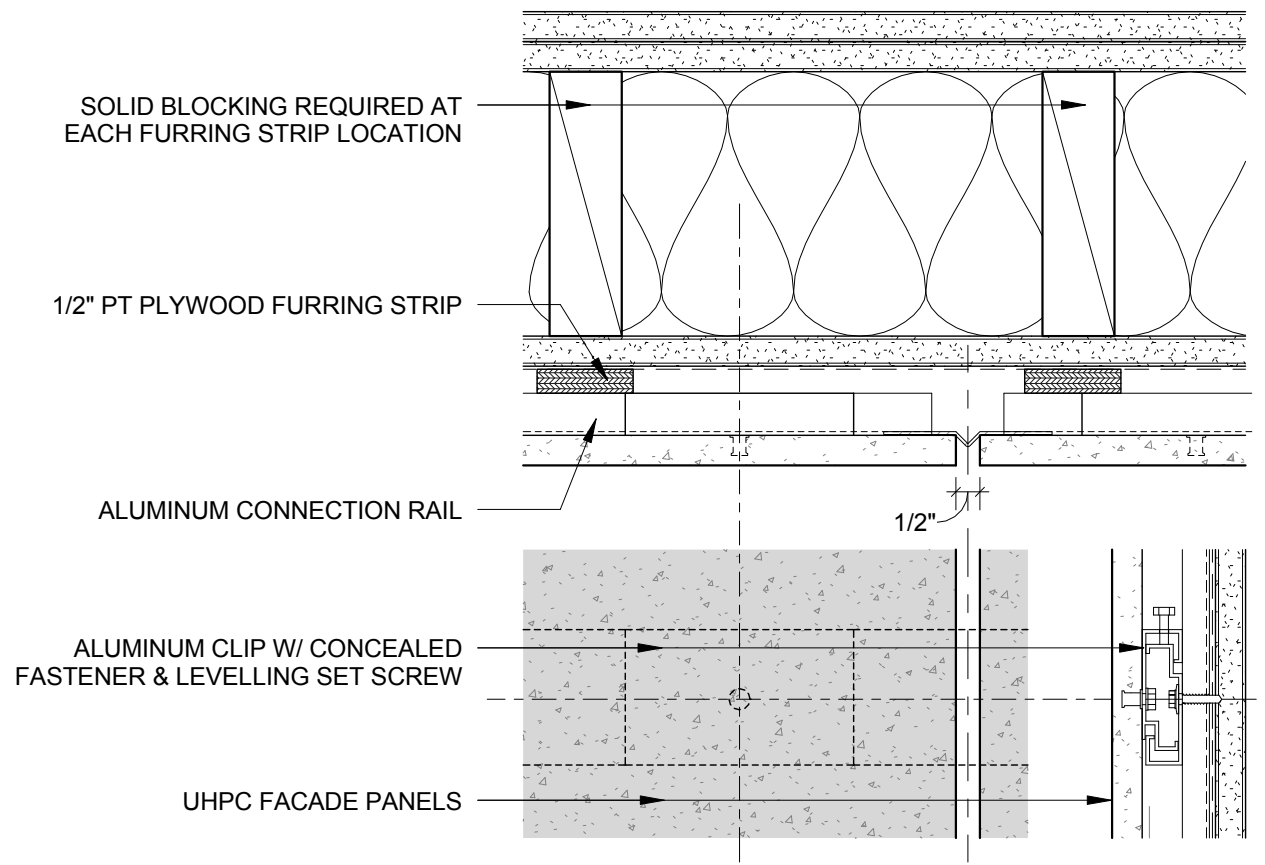
VERTICAL PANEL JOINT
