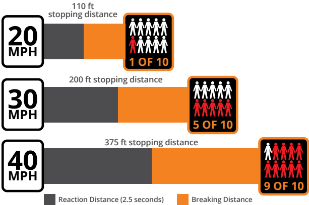
Fig. 3: Effects of Vehicle Speed on Braking Distance and Fatality Rate in Collisions
