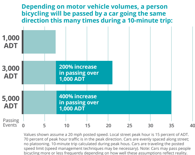
Fig. 4: Performance Guidelines
