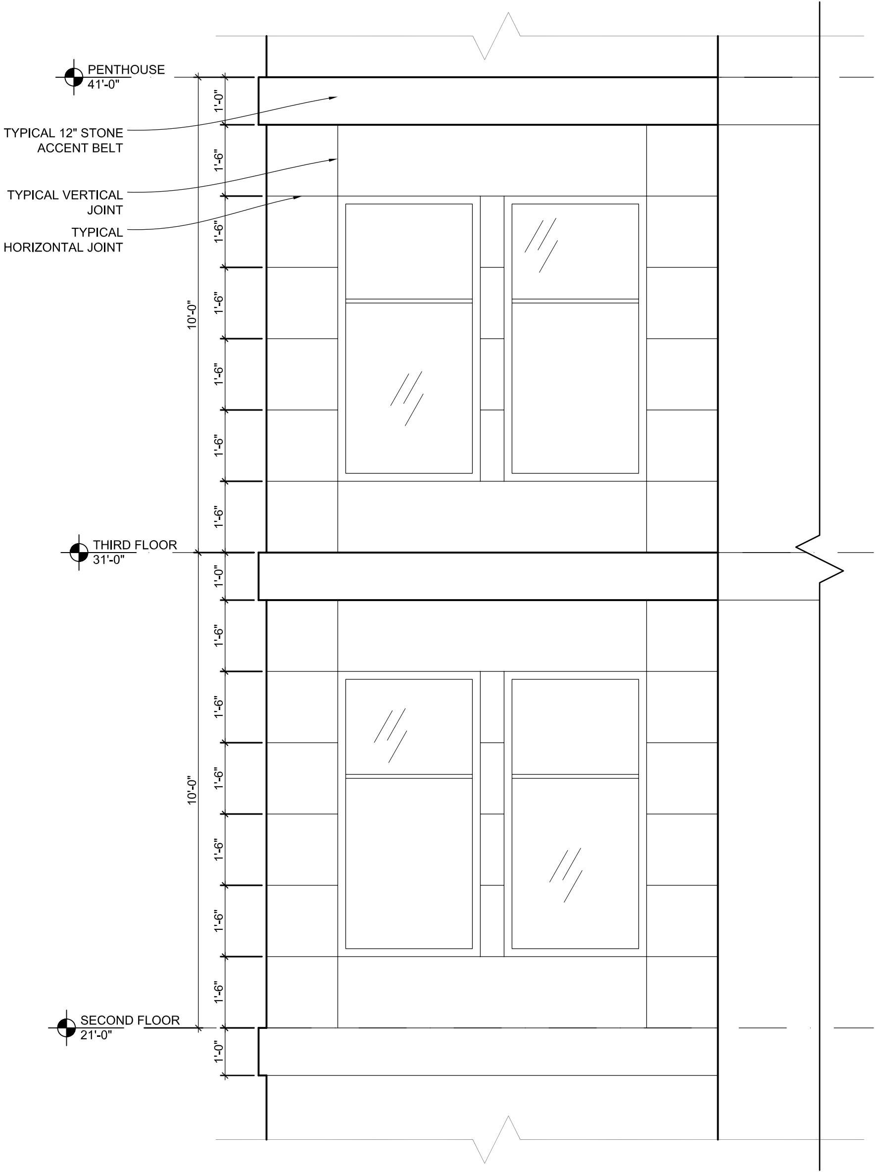
1 PARTIAL ENLARGED ELEVATION AT TYPE-2 STONE
