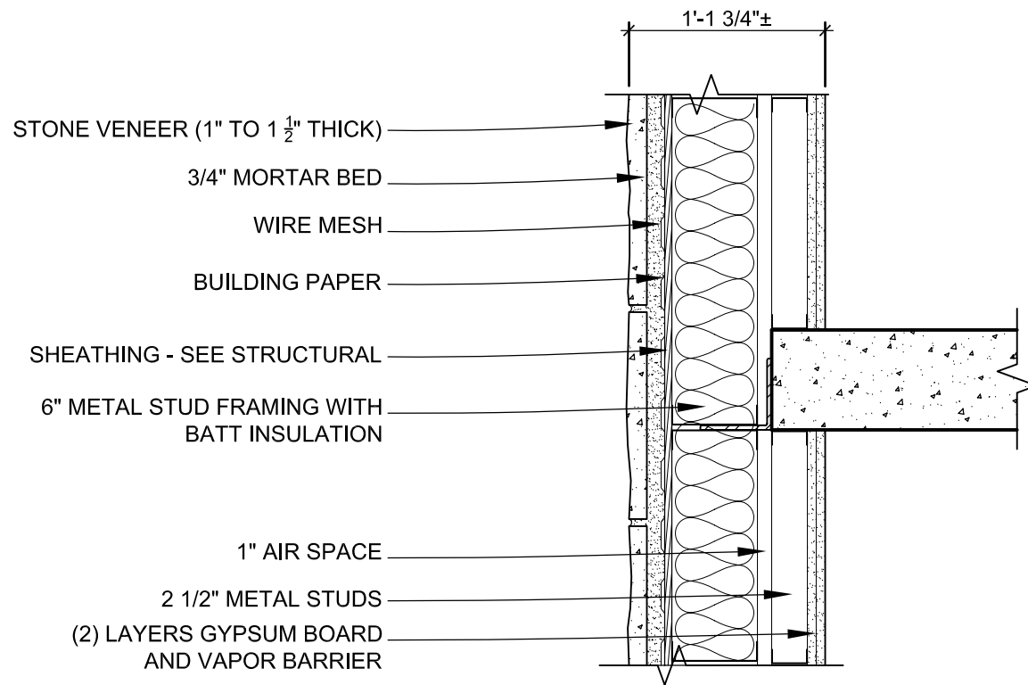
3 DOUBLE METAL STUD WALL 1" = 1'-0"
