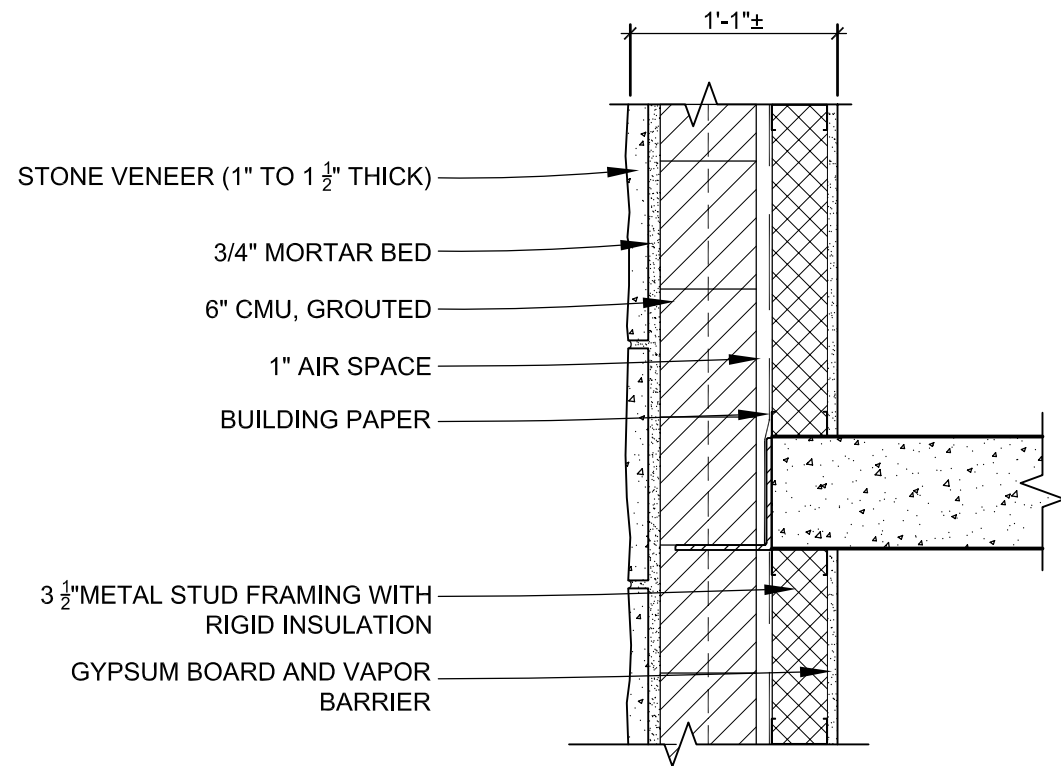
1 SELF SUPPORTING CMU WALL 1" = 1'-0"
