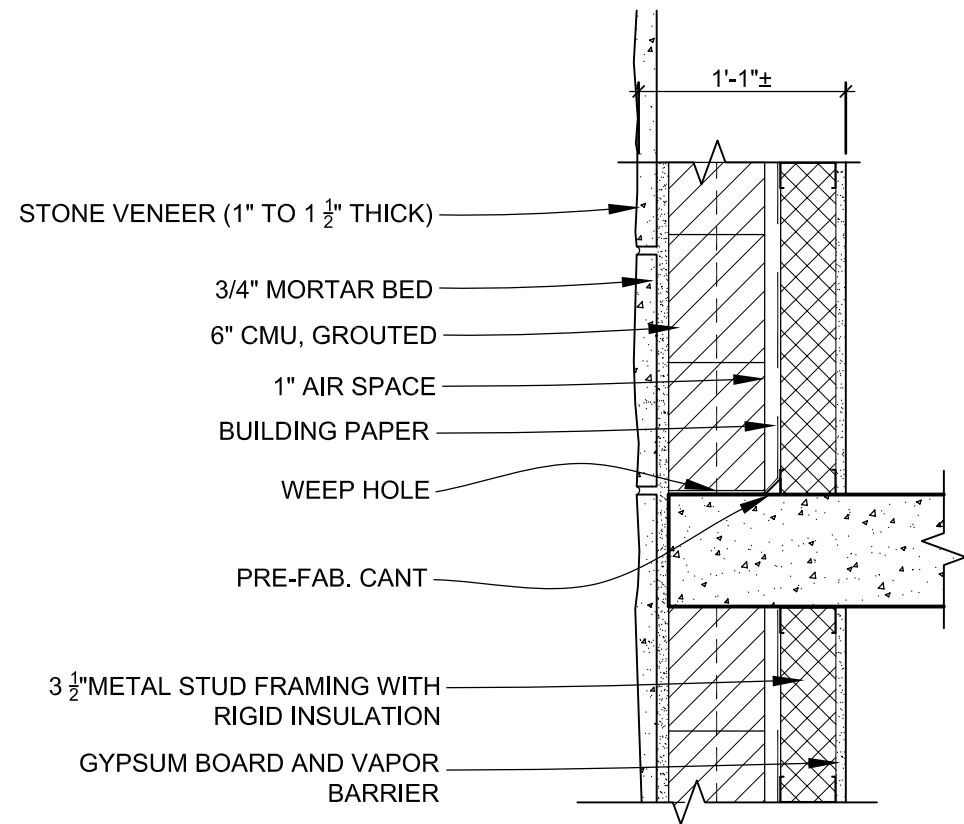
2 CMU WALL - SUPPORTED ON FLOOR SLABS 1" = 1'-0"
