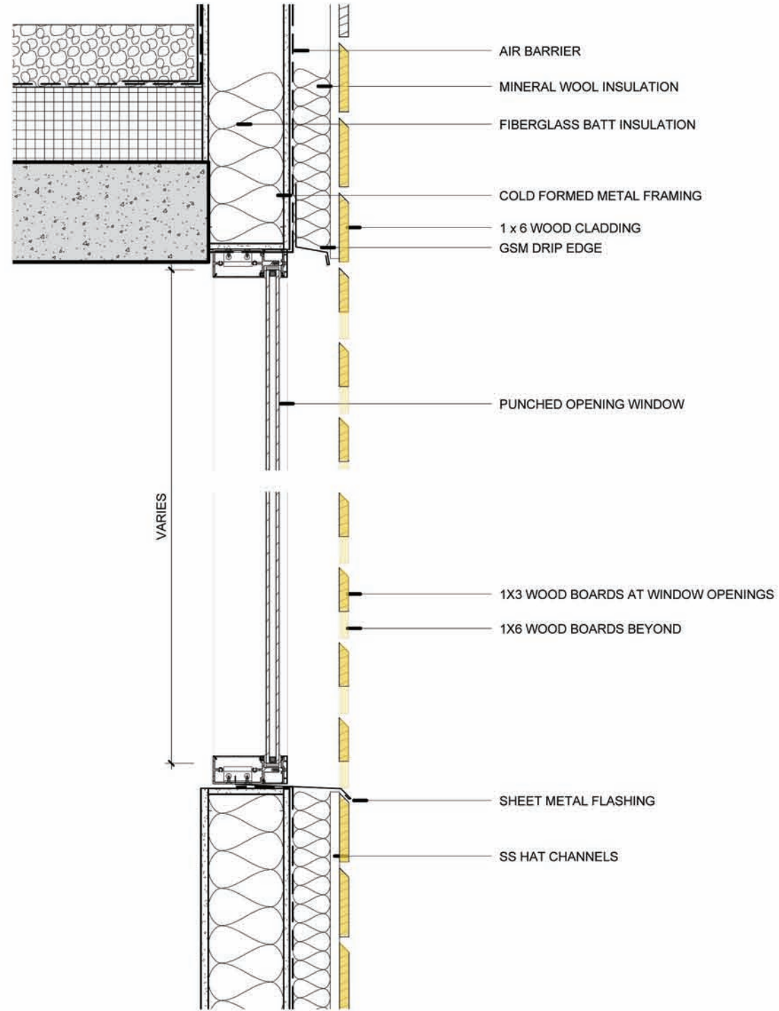
13 Typical Pavilion E/W Screened Window Section A520 1 1/2" = 1'-0"
