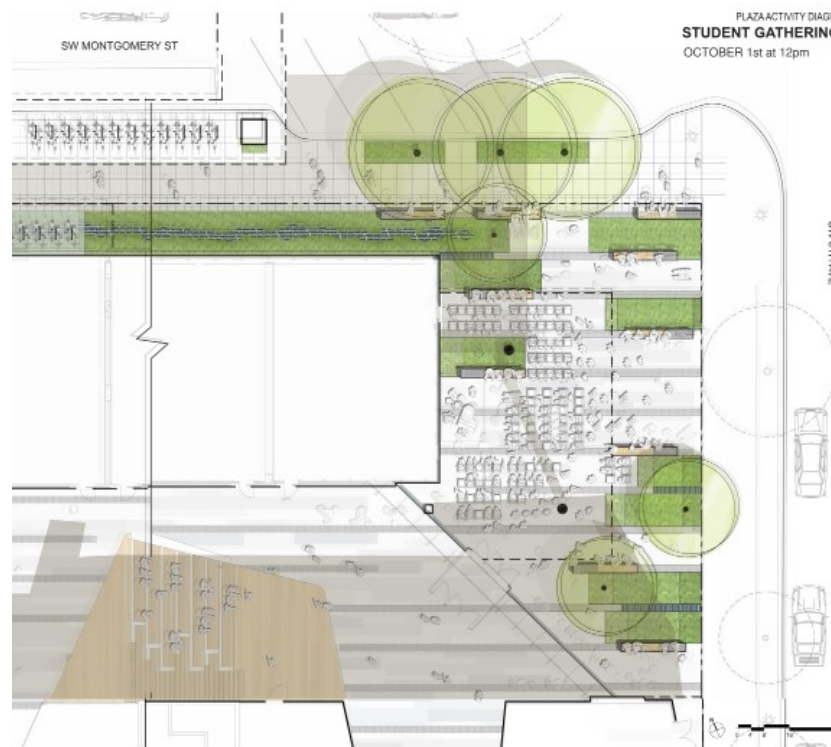
FORECOURT October 1st at 12pm
