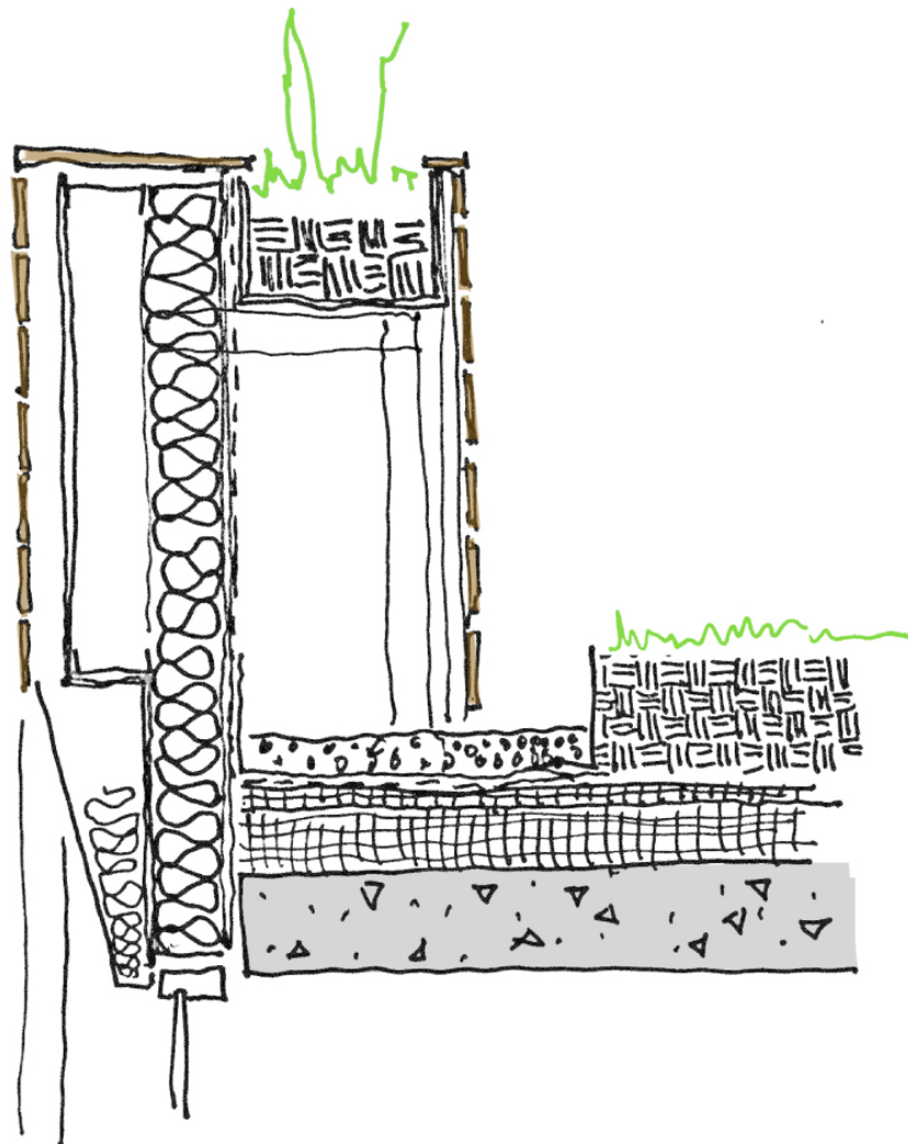
Parapet Planter Section Detail
