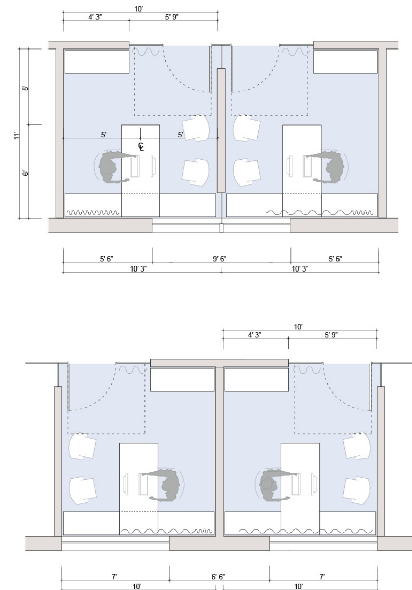
Typical Plan @ Renovation
