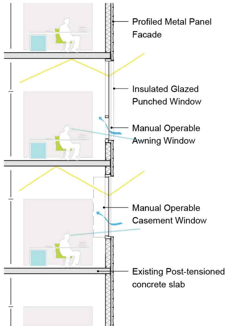
Enlarged Section @ Renovation
