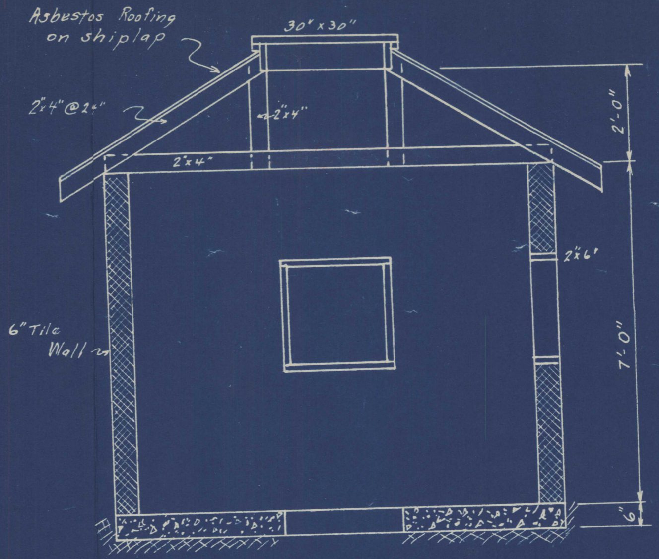
SECTION
