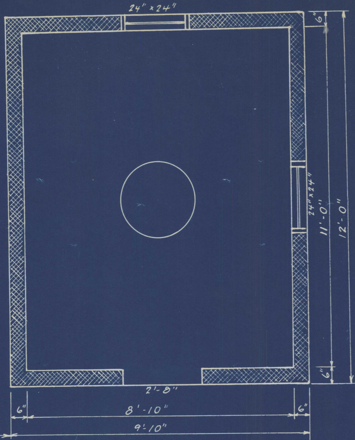
PLAN
