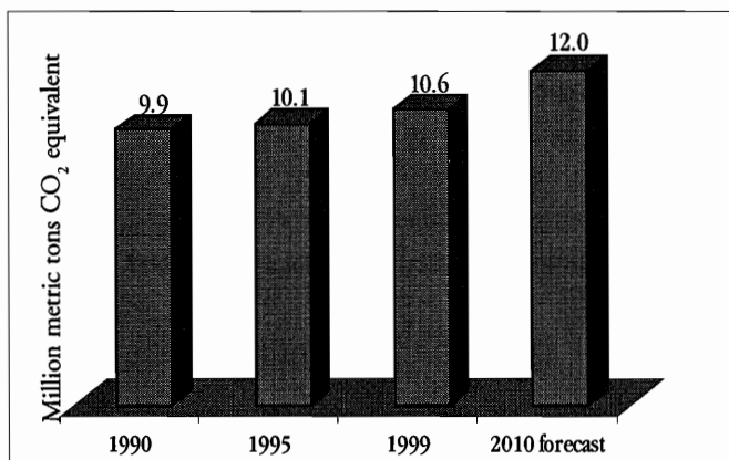
Figure 1. Total Multnomah County greenhouse gas emissions
