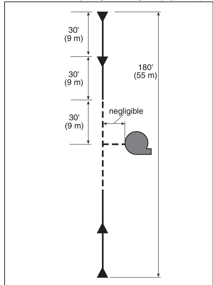
FIGURE 24: Example System Layout (Option 7)
