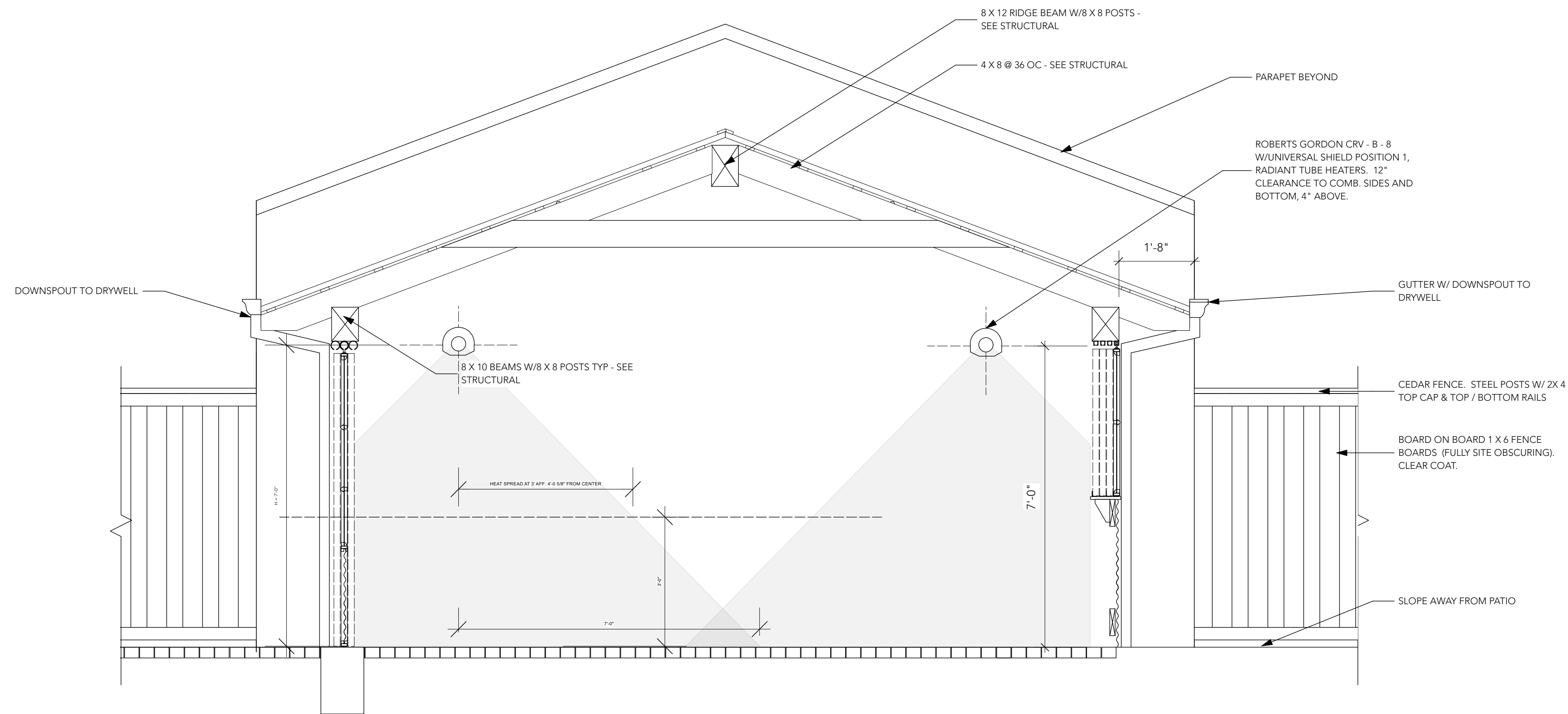
1 SECTION A3.2 1/2" = 1'
