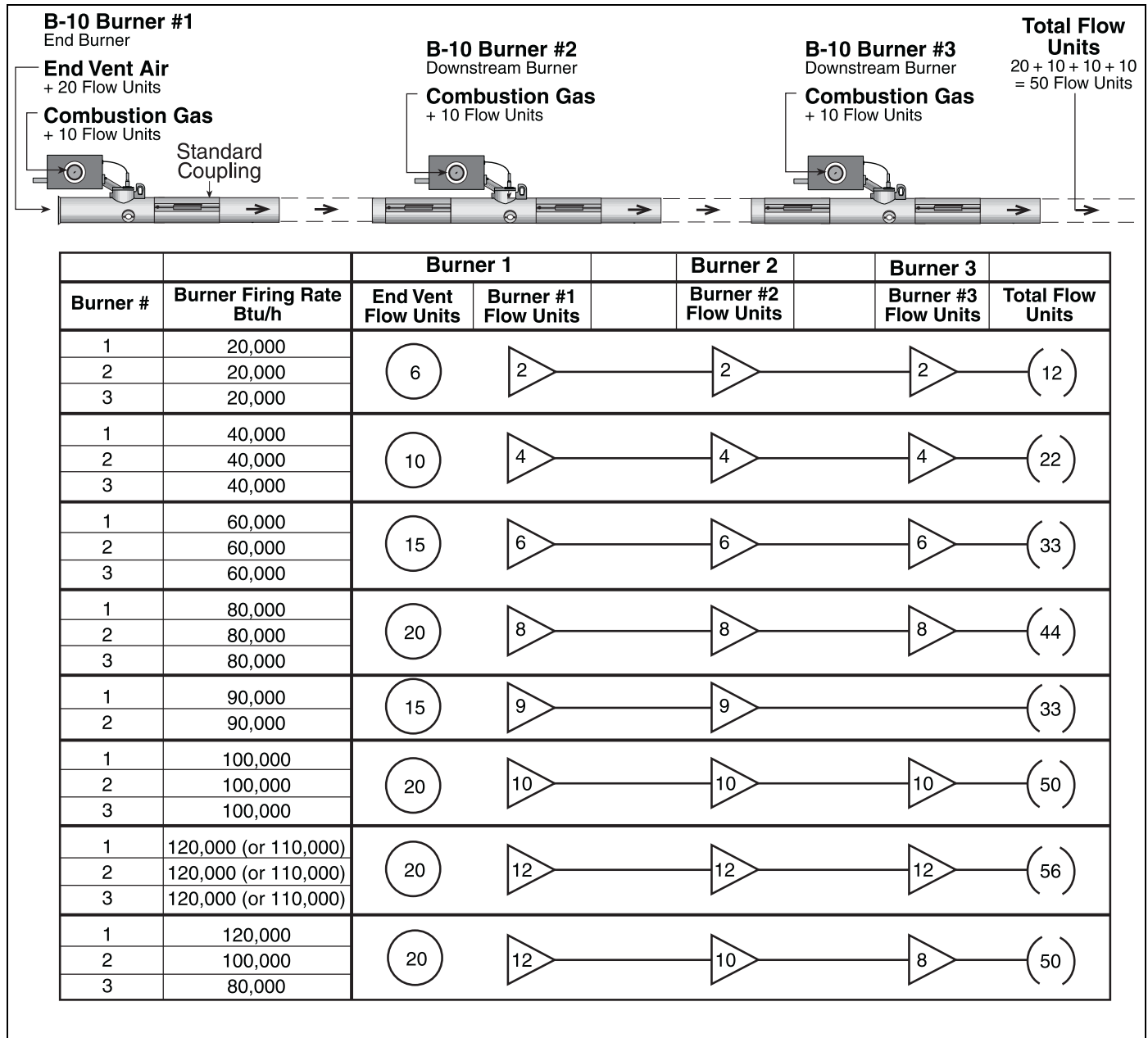
FIGURE 14: Burner Flow Units
