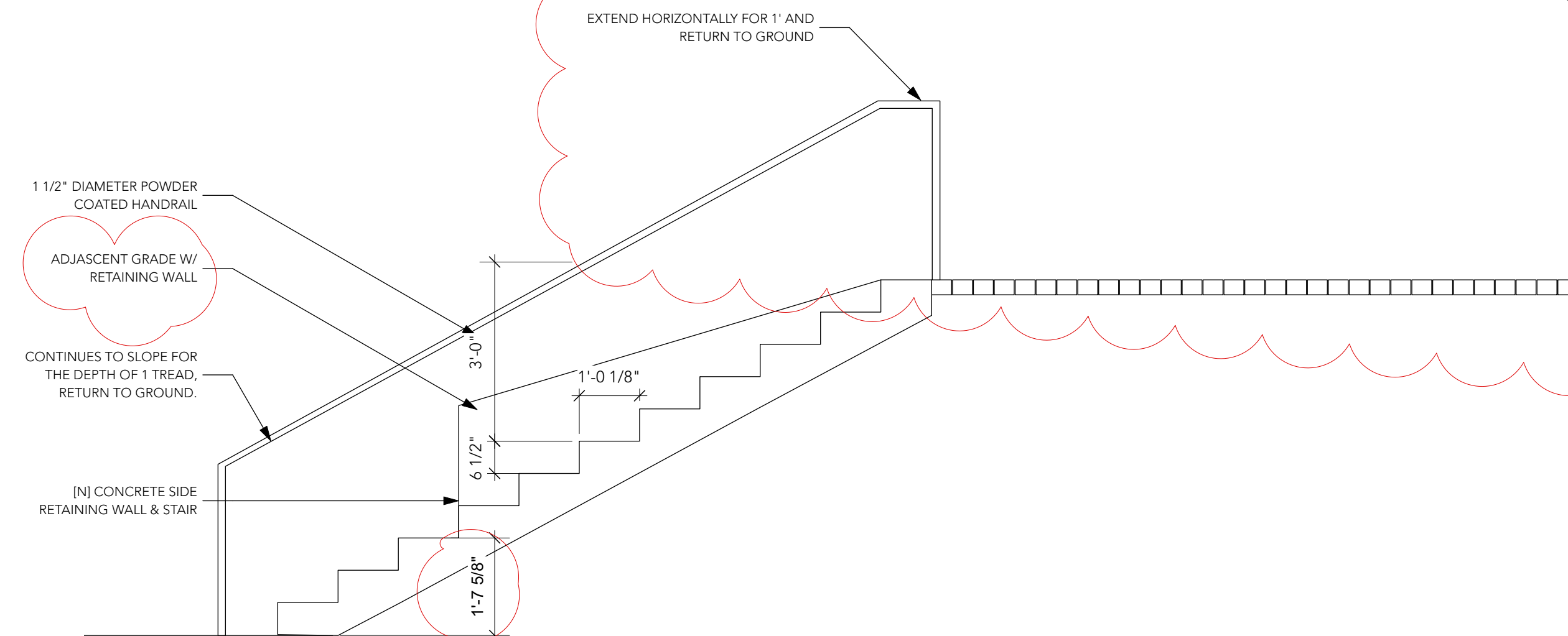
3 SECTION @ STAIR A3.2 1/2" = 1'
