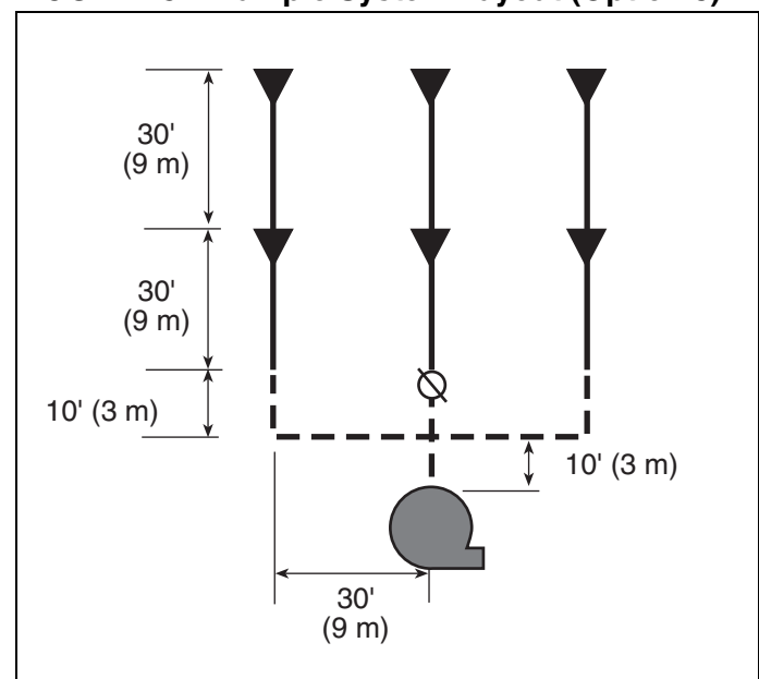
FIGURE 25: Example System Layout (Option 8)
