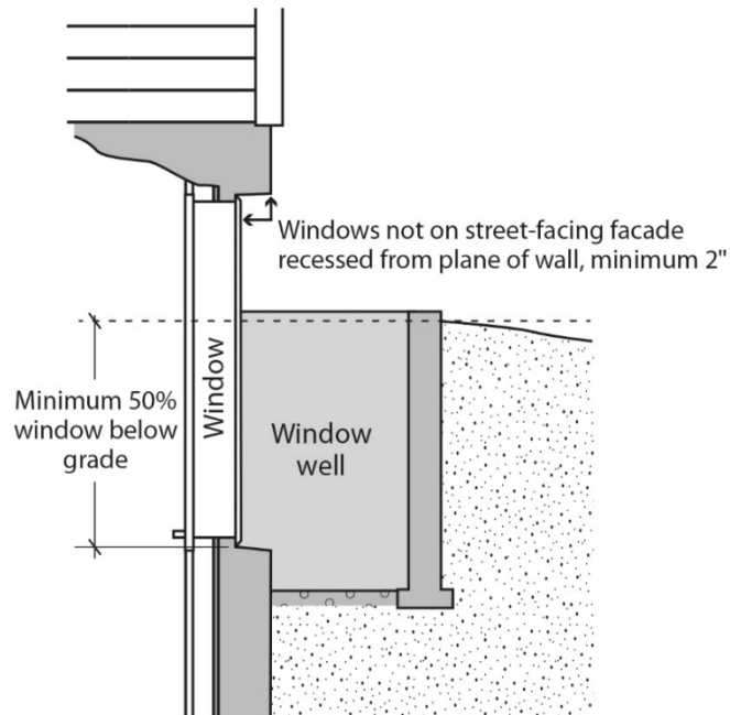
Figure 445-4 Basement Windows
