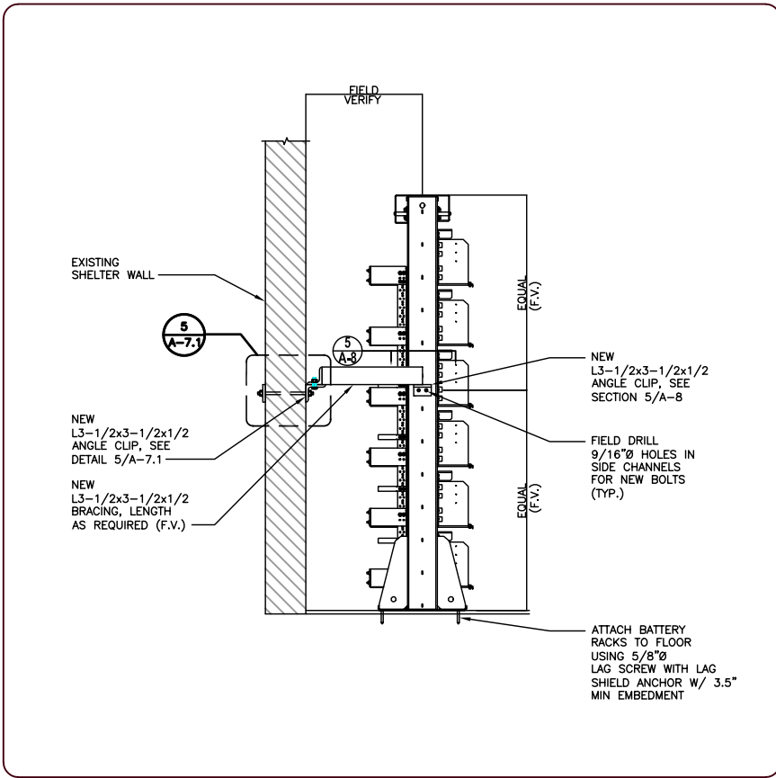
4 SECTION DETAIL A-7.1 SCALE: NTS
