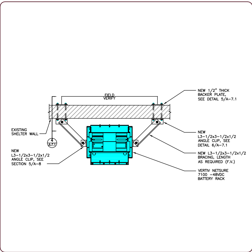
2 PROPOSED VERTIV NETSURE-48VDC PLAN DETAIL A-7.1 SCALE: NTS
