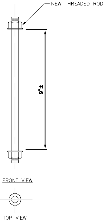
2 THREADED ROD DETAIL A-7.2 SCALE: NTS
