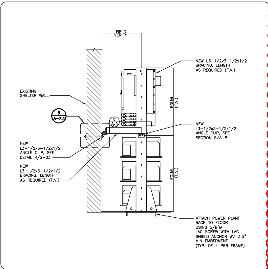
3 SECTION DETAIL A-7.1 SCALE: NTS
