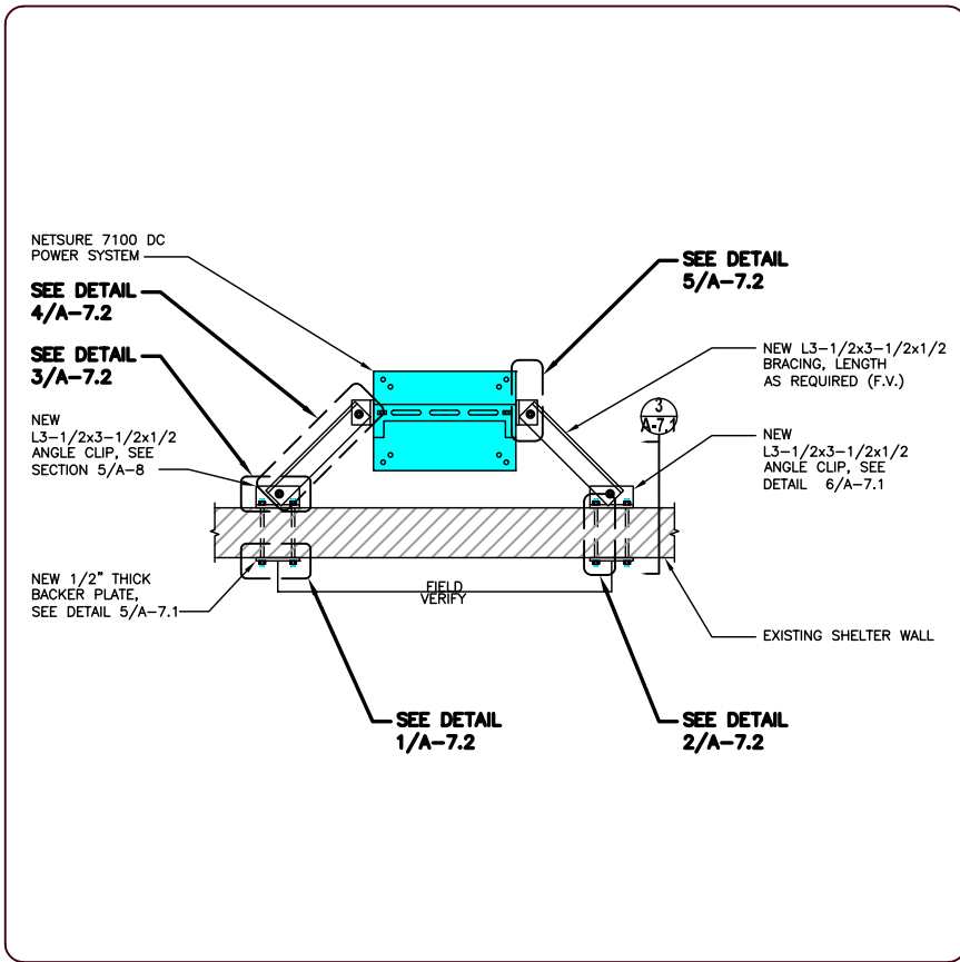
1 PROPOSED NETSURE 7100 DC PLAN DETAIL A-7.1 SCALE: NTS
