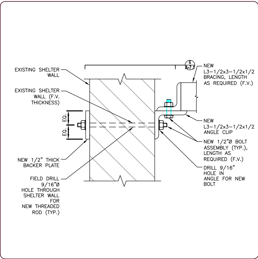
5 CLIP DETAIL A-7.1 SCALE: NTS
