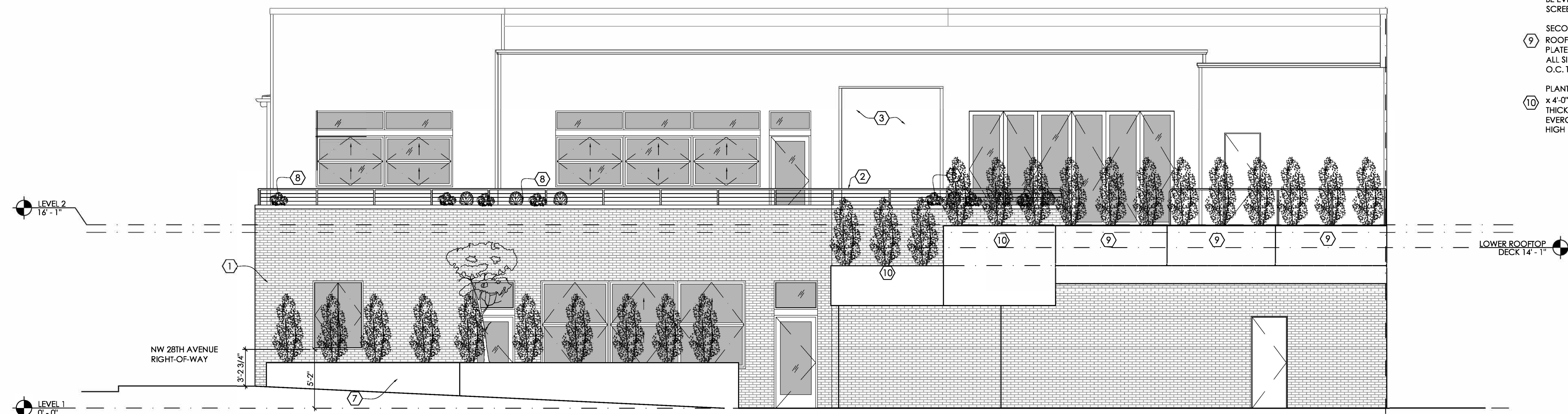
2 SOUTH ELEVATION 3/16" = 1'-0"
