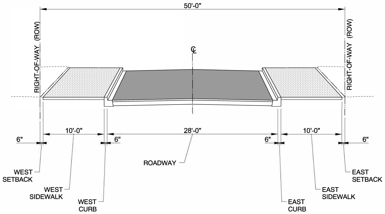
PARK TYPICAL SECTION
