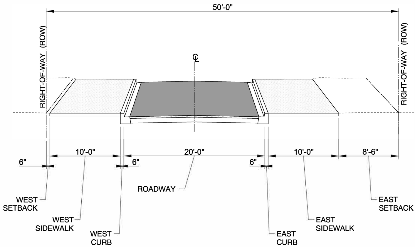
NON-PARK TYPICAL SECTION
