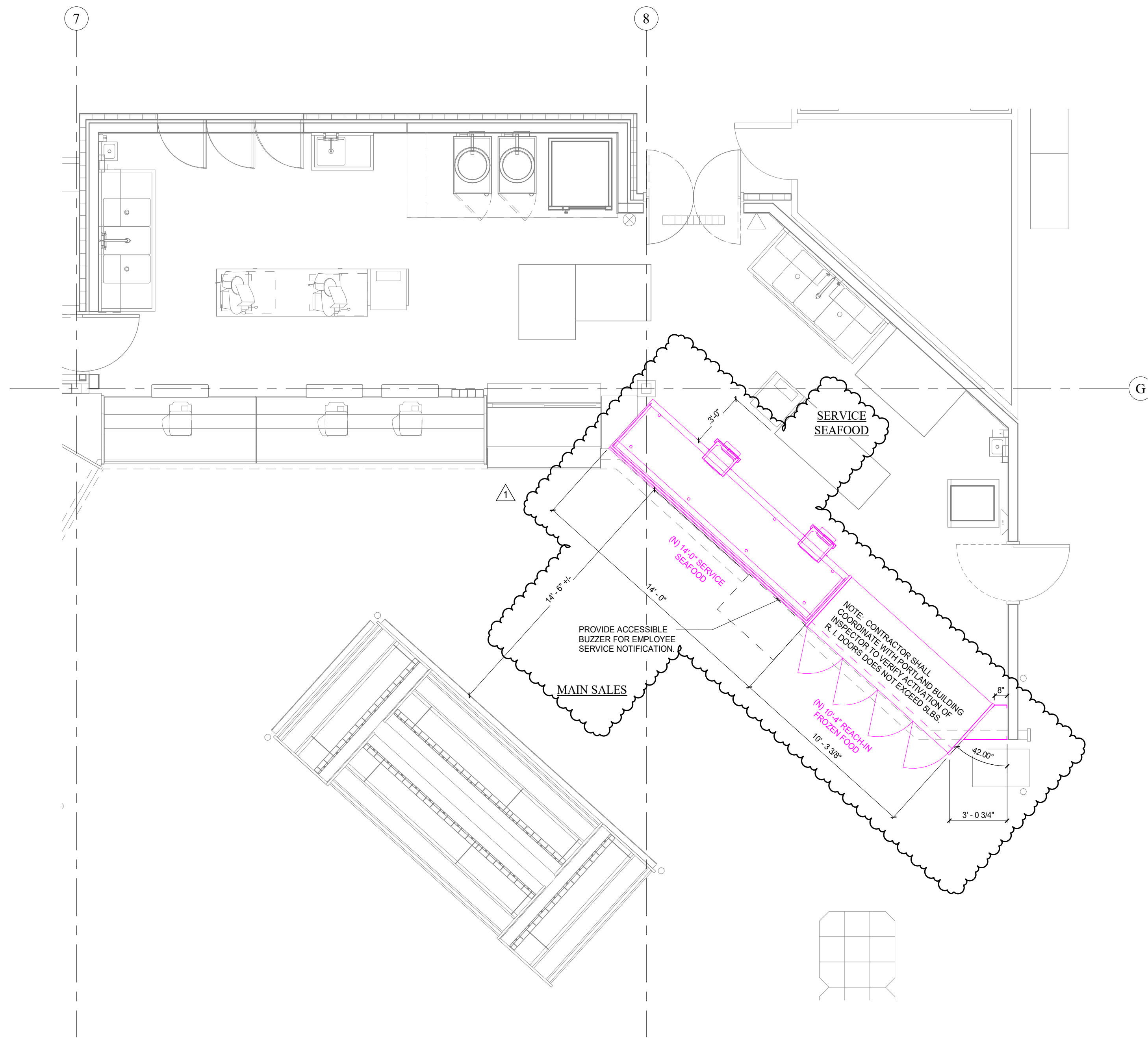
ENLARGED SERVICE SEAFOOD PLAN 1/4" = 1'-0"
