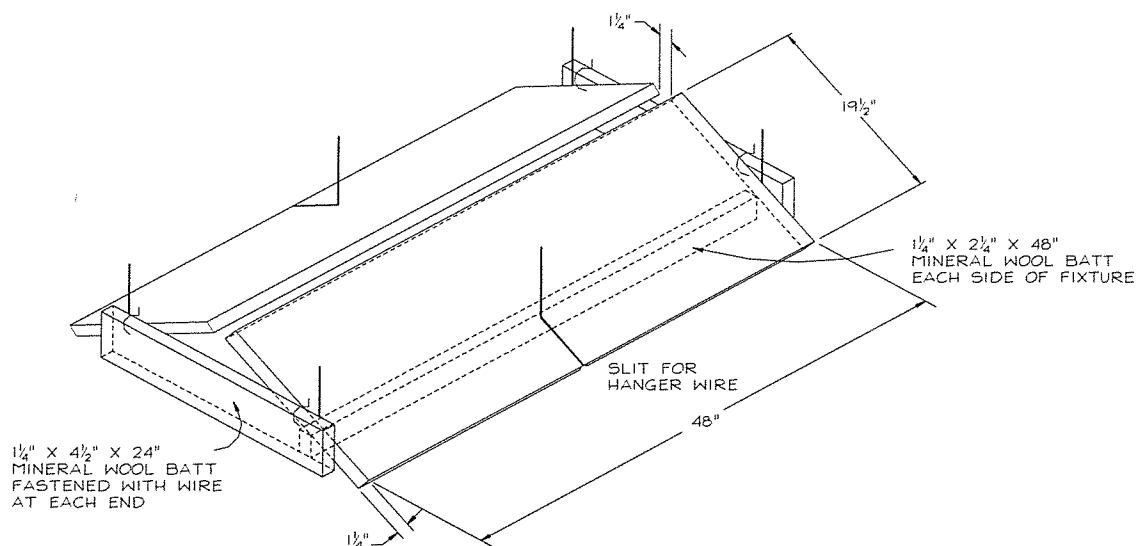
FIGURE 4—LIGHT FIXTURE PROTECTION
