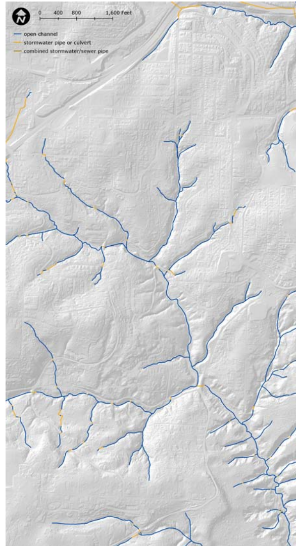
Remapped Centerlines
