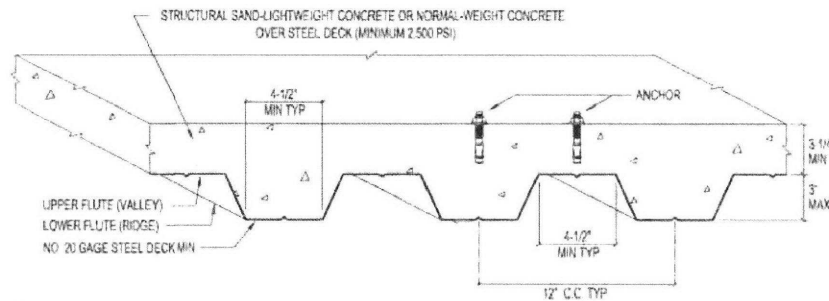
Figure 1 - Power-Stud+ SD1 Installation Detail for Anchors in the Topside Of Concrete-Filled Steel Deck Floor and Roof Assemblies (See Dimensional Profile Requirements)
