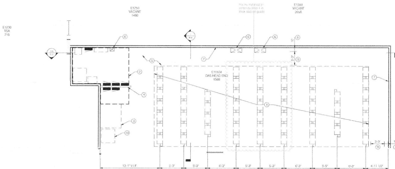
1 DEPLANING LEVEL - EQUIPMENT PLAN SCALE: 1/4" = 1'-0"
