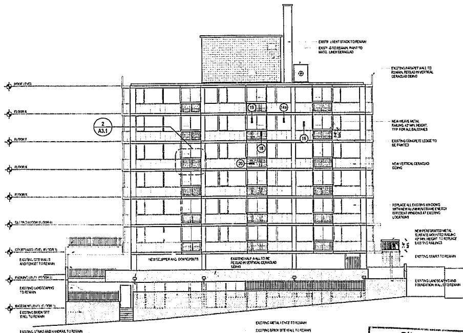
② EAST ELEVATION SCALE 1/8" = 1'-0"
