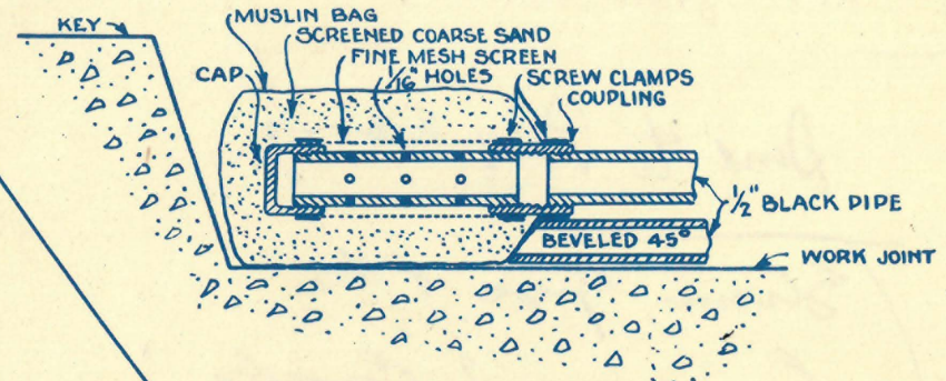
DETAILS OF UPLIFT POINT SCALE ~ 1" = 4"
