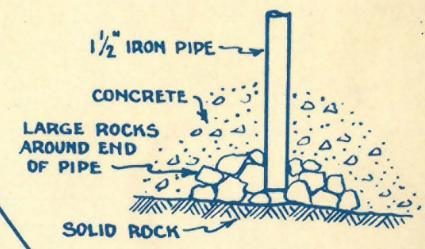
UPLIFT POINT TYPE A, A 2 , B, B 2 NO SCALE
