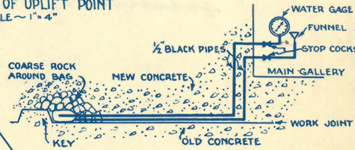
UPLIFT POINT CONNECTIONS NO SCALE
