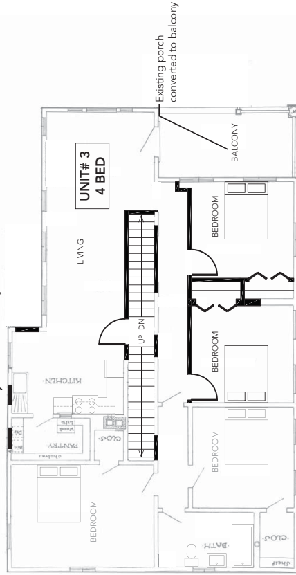
PLAN 2nd Level 1,595 sf
