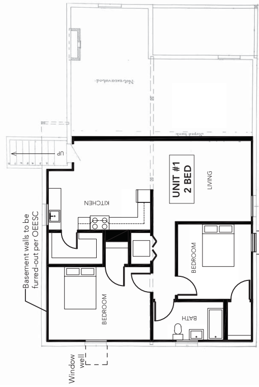
PLAN Basement 1,095 sf
