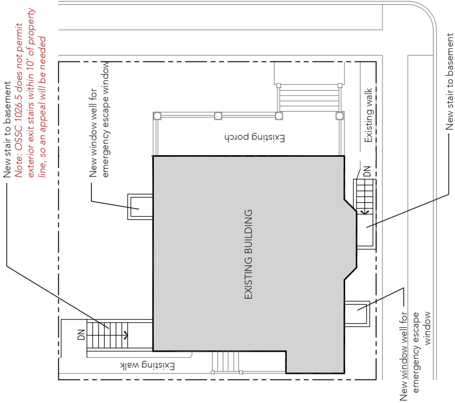
SITE PLAN
