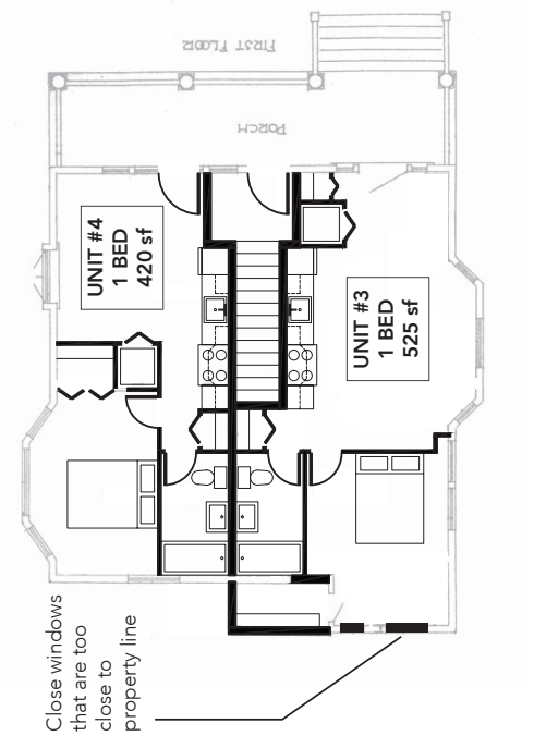
PLAN 1st Level 1,000 sf
