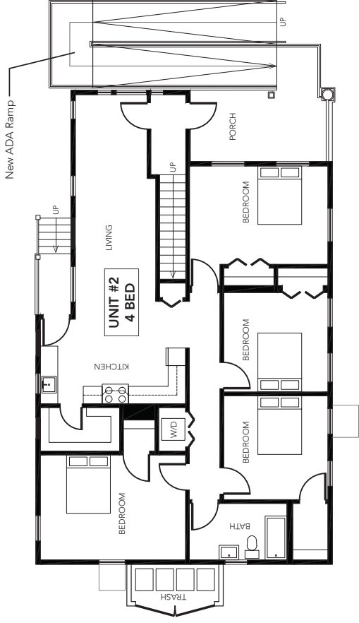
PLAN 1st Level 1,595 sf
