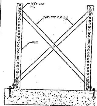
(3) "X" BRACING DETAIL
