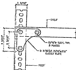
(1) SHELF CONNECTION
