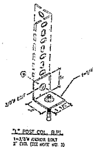
(2) BASE PLATE DETAIL
