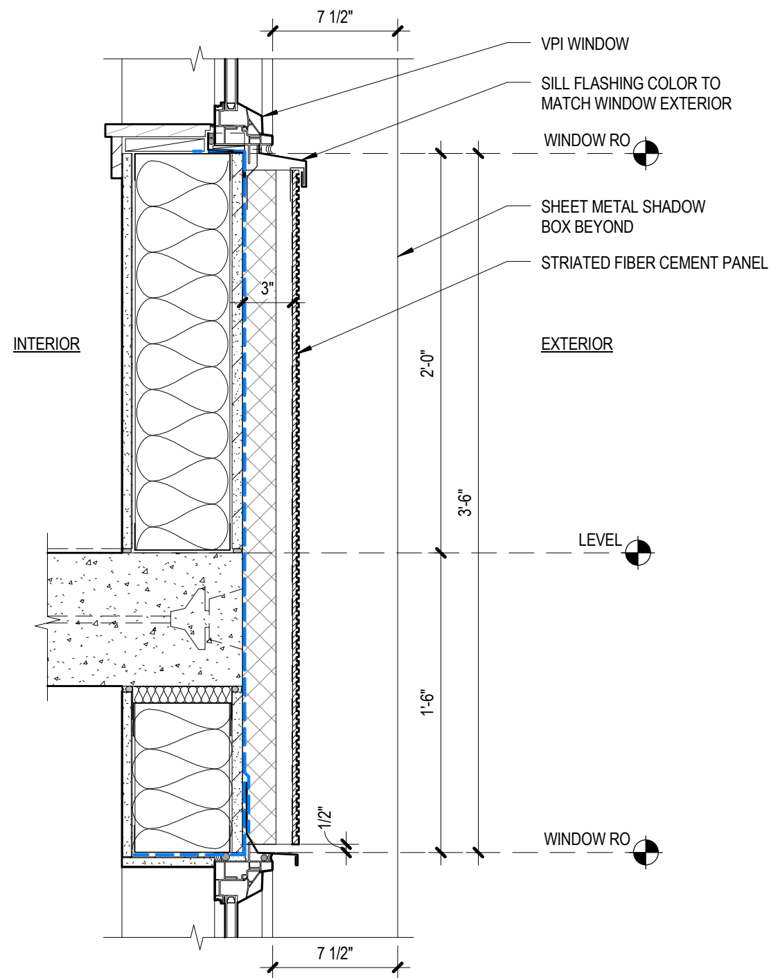
WINDOW HEAD/SILL @ SHALLOW WALL
