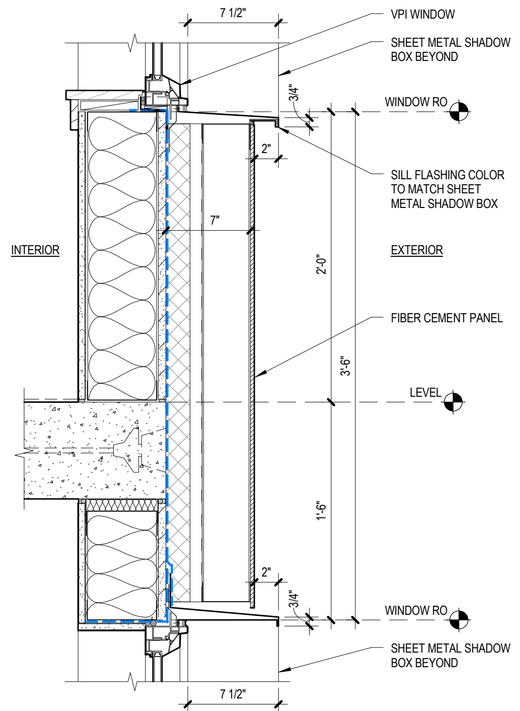
WINDOW HEAD/SILL @ DEEP WALL
