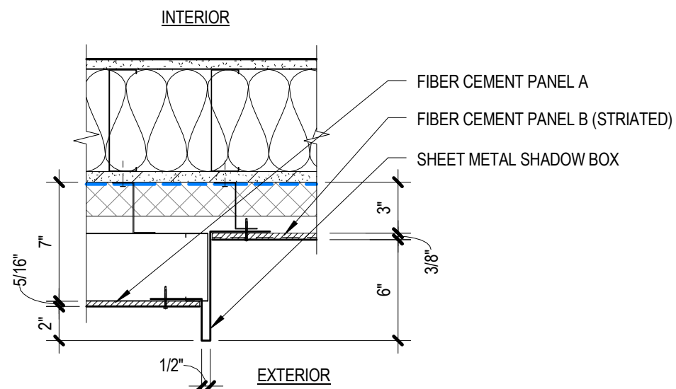
3 FIBER CEMENT TRANSITION
