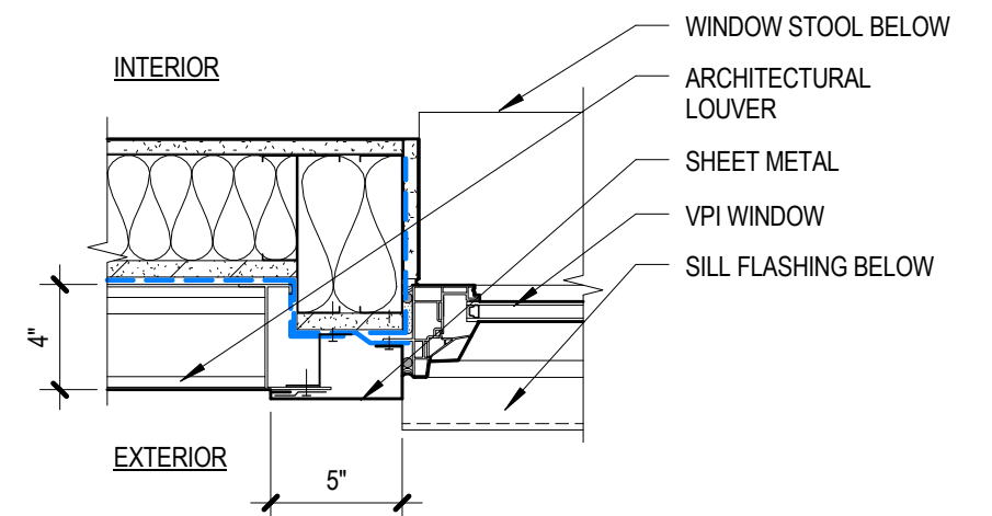
2 WINDOW JAMB @ LOUVER
