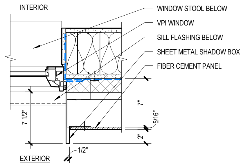
4 WINDOW JAMB, TYP.
