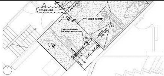
1 ENLARGED SLAB PLAN - RESTROOM AND LOBBY
