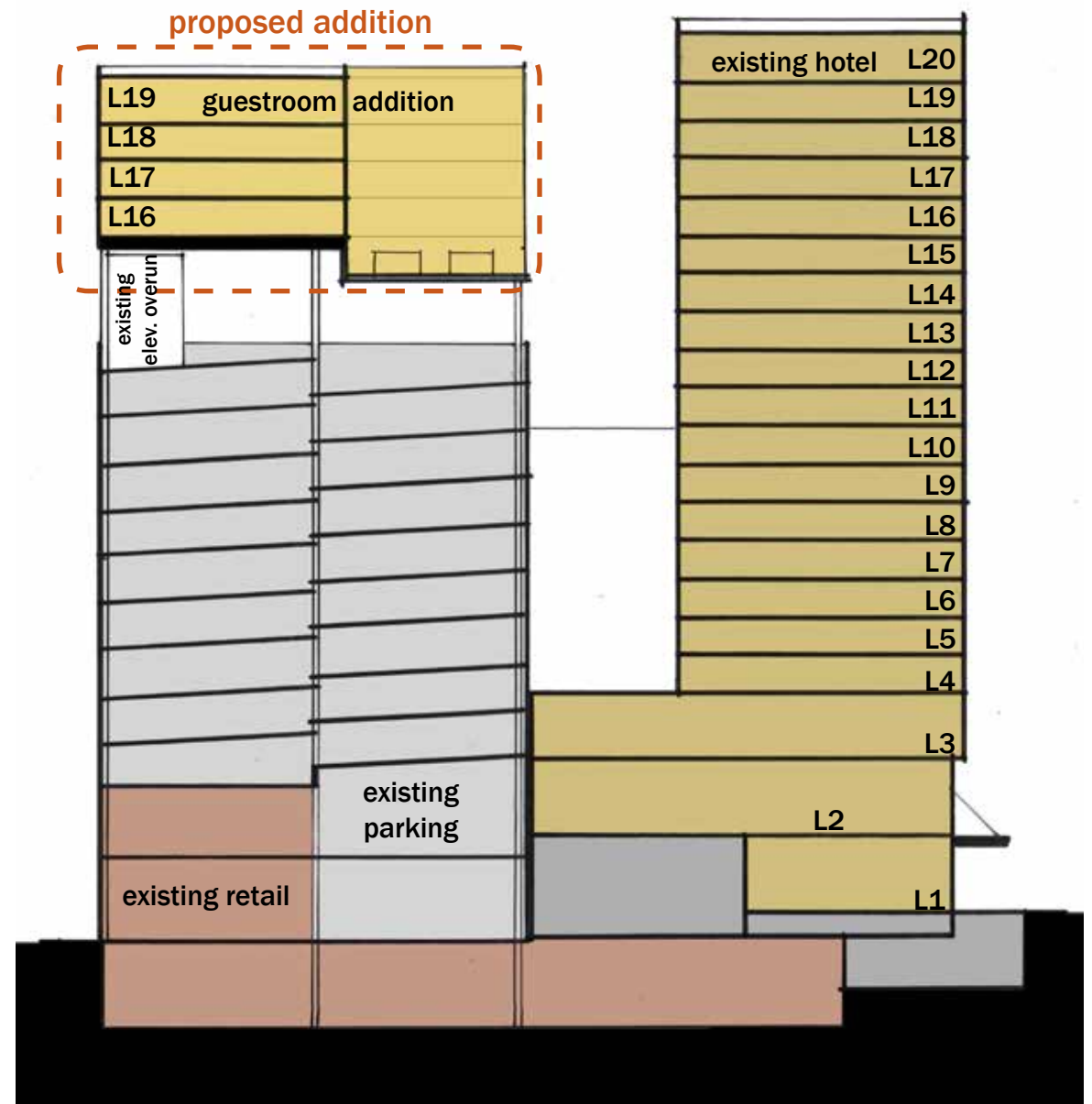
section 2 - proposed
