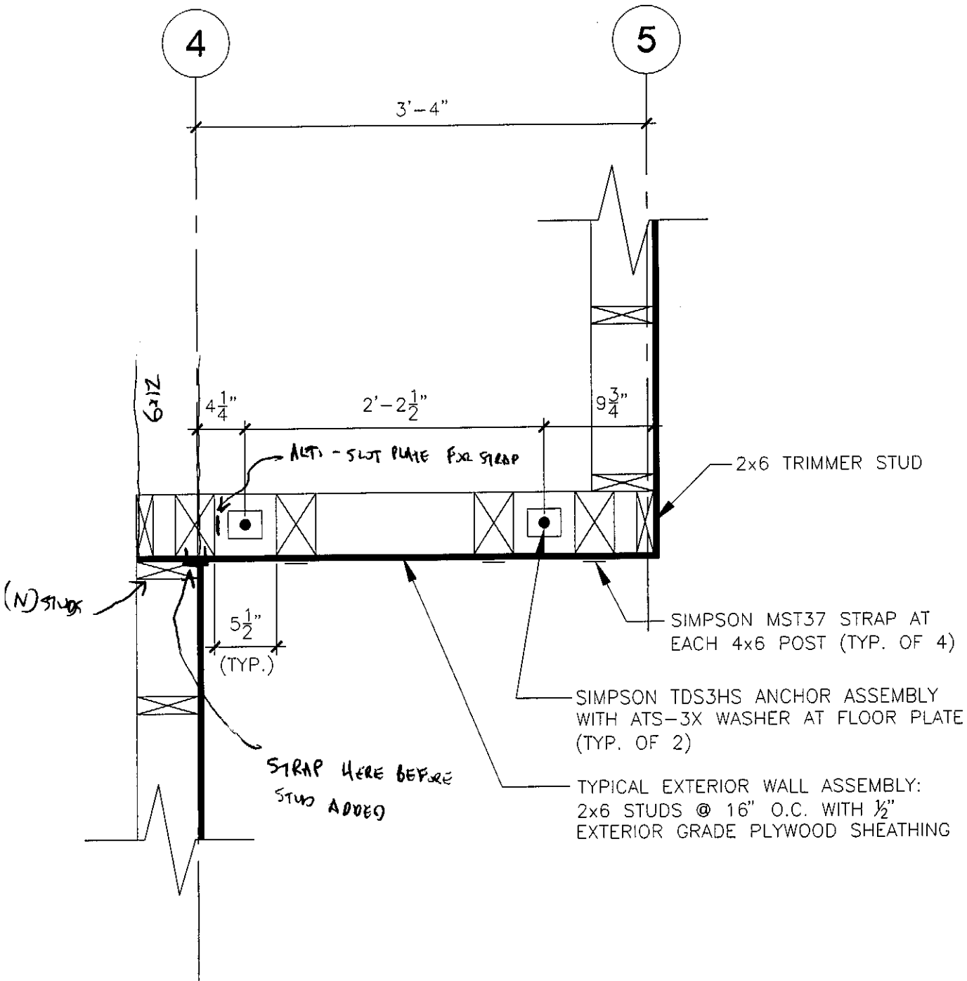
1 TDS ANCHOR PLAN DETAIL - SECOND FLOOR SCALE: N.T.S.
