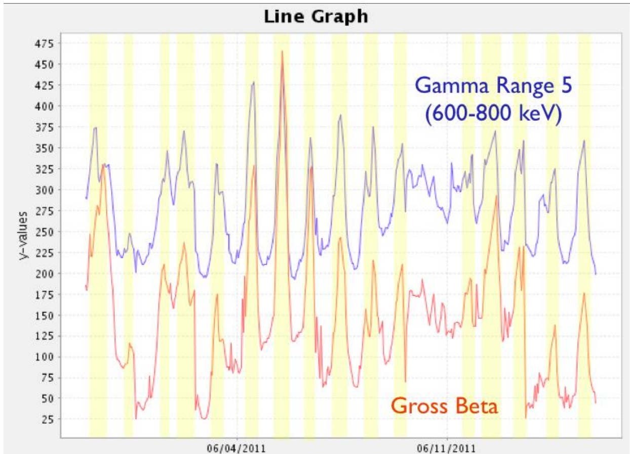
Concurrent radioactive beta \beta and gamma \Gamma activity from radon 222 progeny
