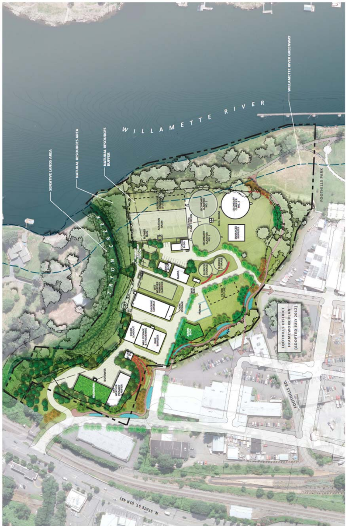
Figure 6.11. Tryon Creek Wastewater Treatment Plant Recommended Site Plan
