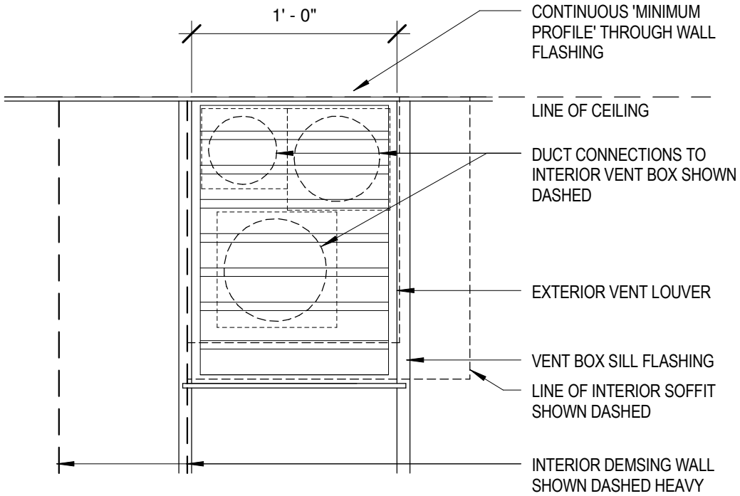
ELEVATION- RESIDENTIAL EXHAUST VENT
