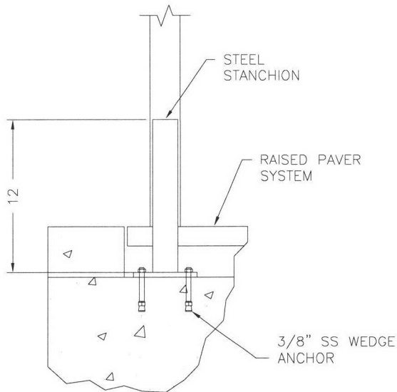
— STANCHION MOUNTING DETAIL SCALE: 3
