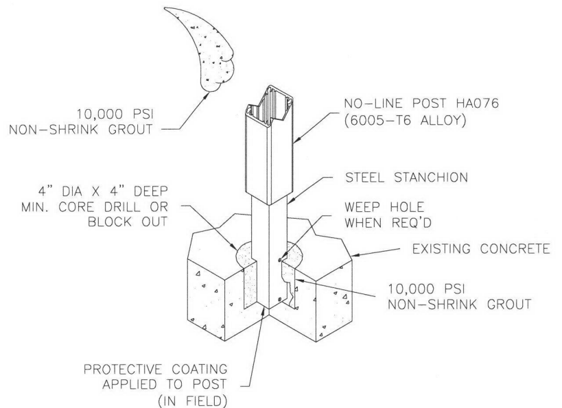
— STANCHION MOUNTING DETAIL CORE POCKET OPTION SCALE: 3
