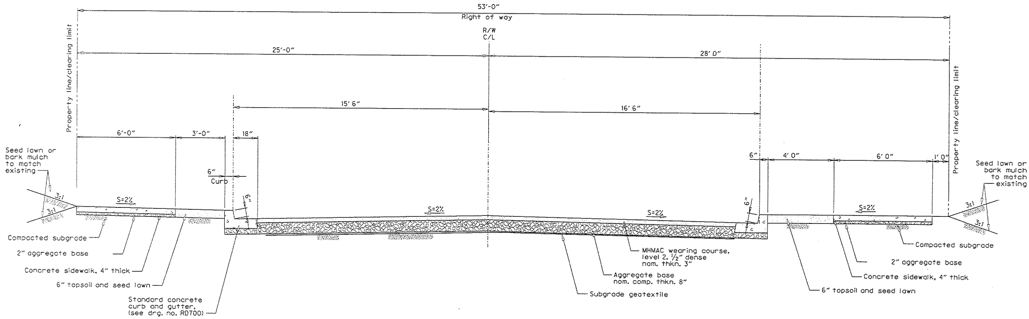
South Typical Section 1 3
