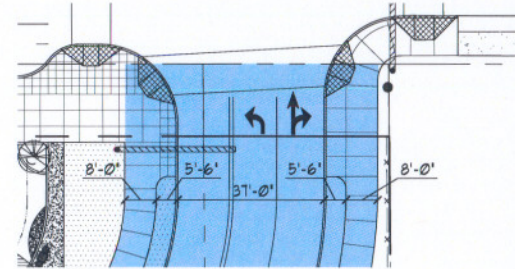
PARTIAL SITE PLAN
