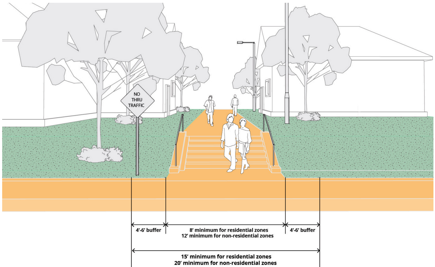
Figure B-34: Pedestrian/Bicycle Connection - stairway
