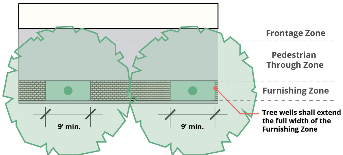
Figure B-12: Tree planting in tree wells
