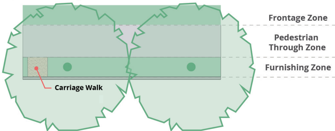
Figure B-11: Tree well and continuous planting strip configuration
