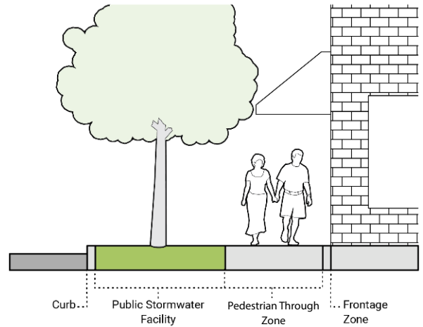
Figure B-8: Furnishing Zone requirements for stormwater facilities
