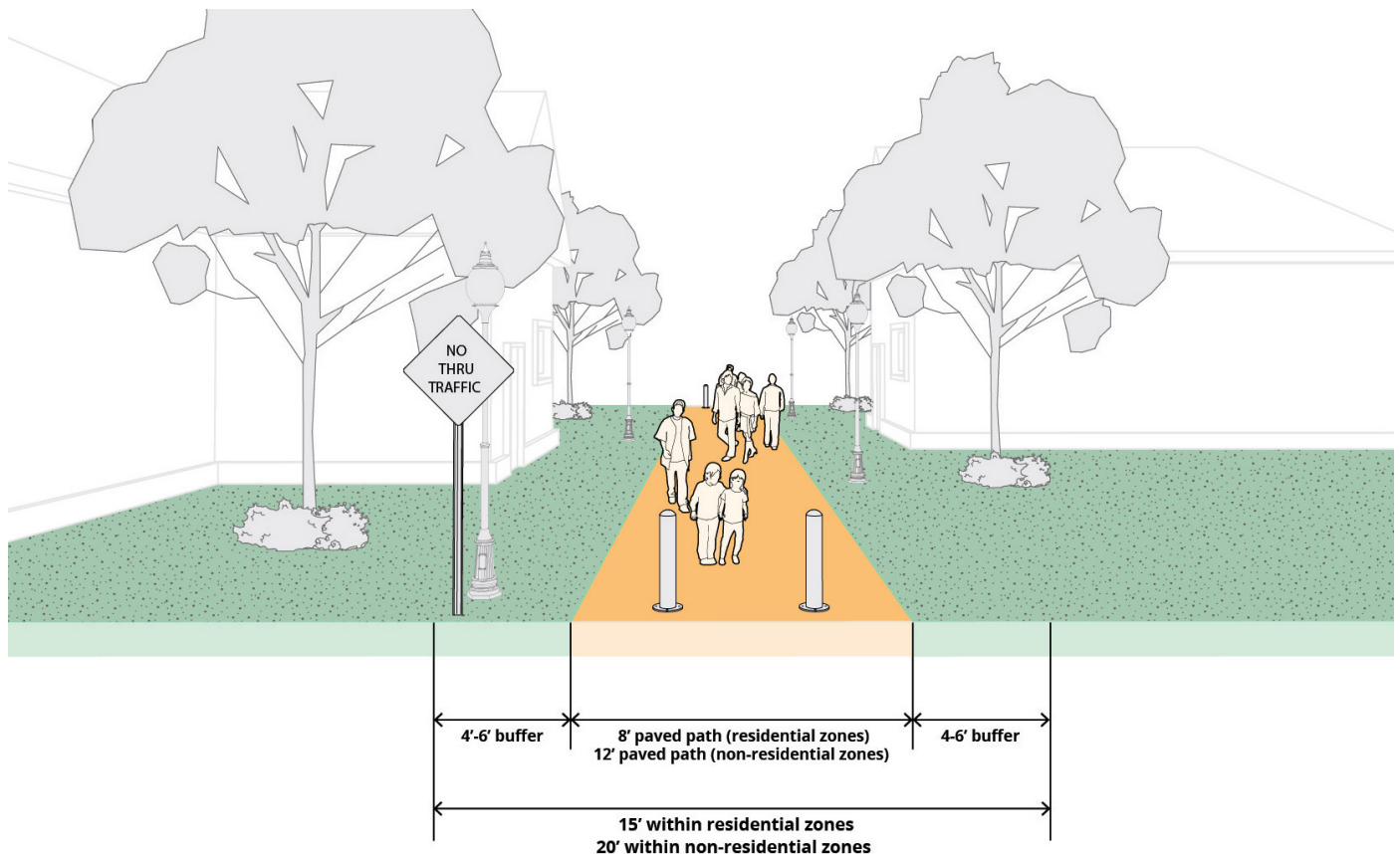
Figure B-32: Pedestrian/Bicycle Connection
