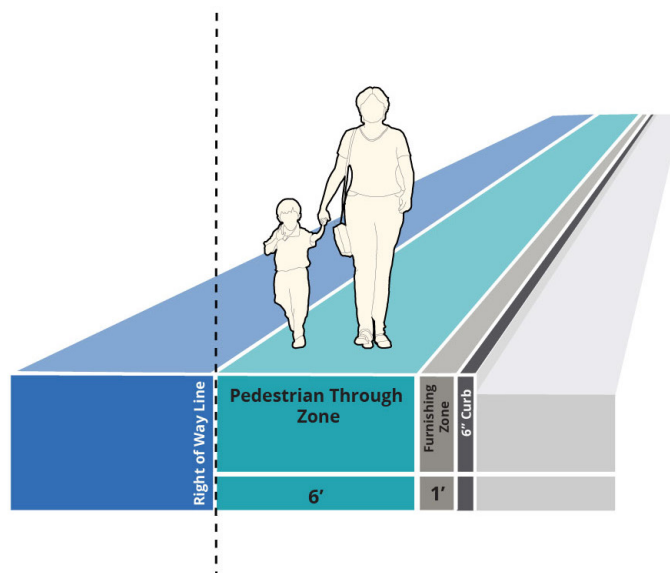
Figure B-24: Curb-tight sidewalk zone widths
