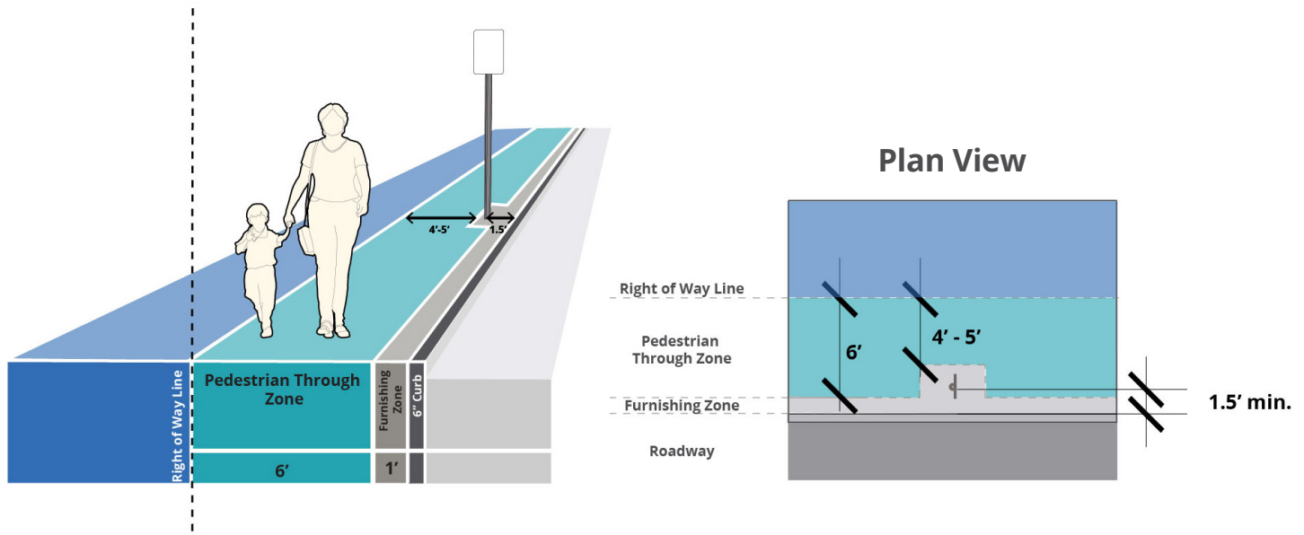
Figure B-25: Pinch point schematic for curb-tight sidewalk corridors
