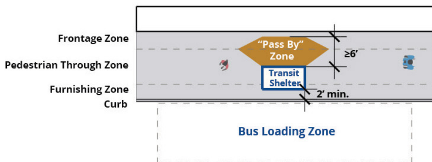
Figure B-14: Transit shelter placement on sidewalk corridors
