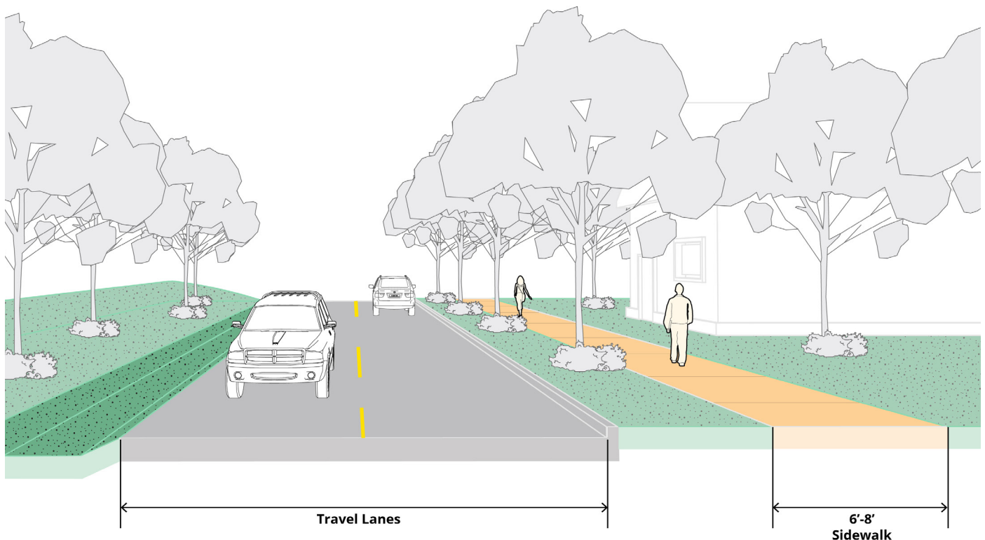
Figure B-30: Sidewalk on One Side of Roadway
