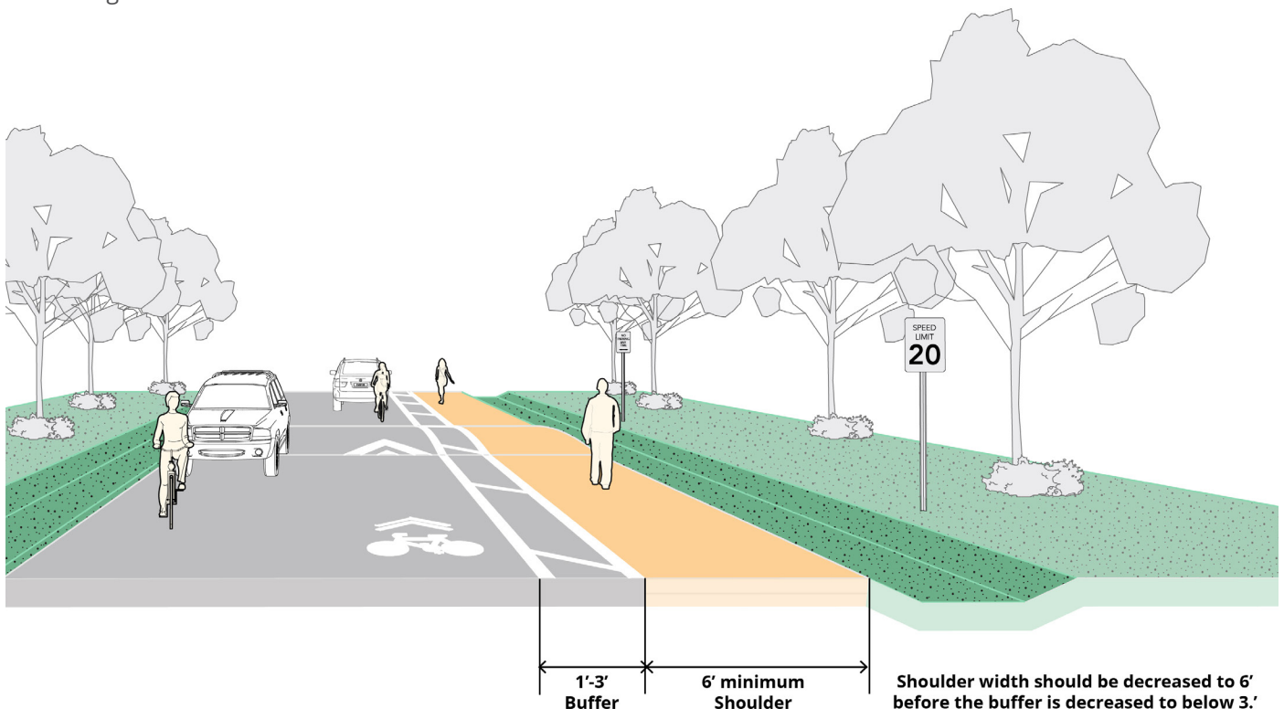
Figure B-38: Slow Safer Shoulder
