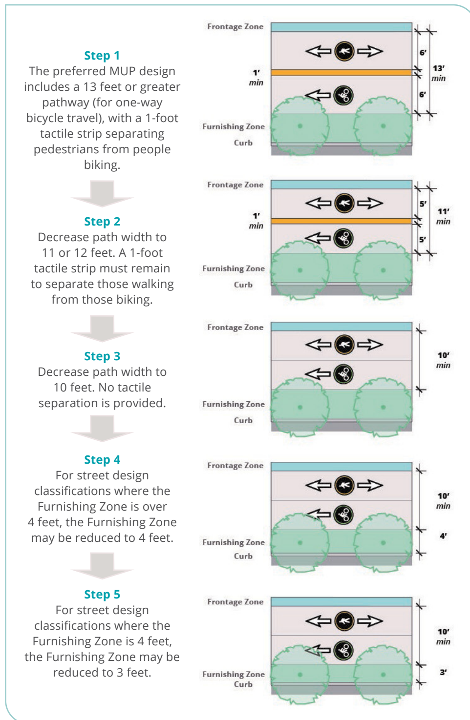
Figure B-22: Process for allocating multi-use path zone widths in constrained conditions
