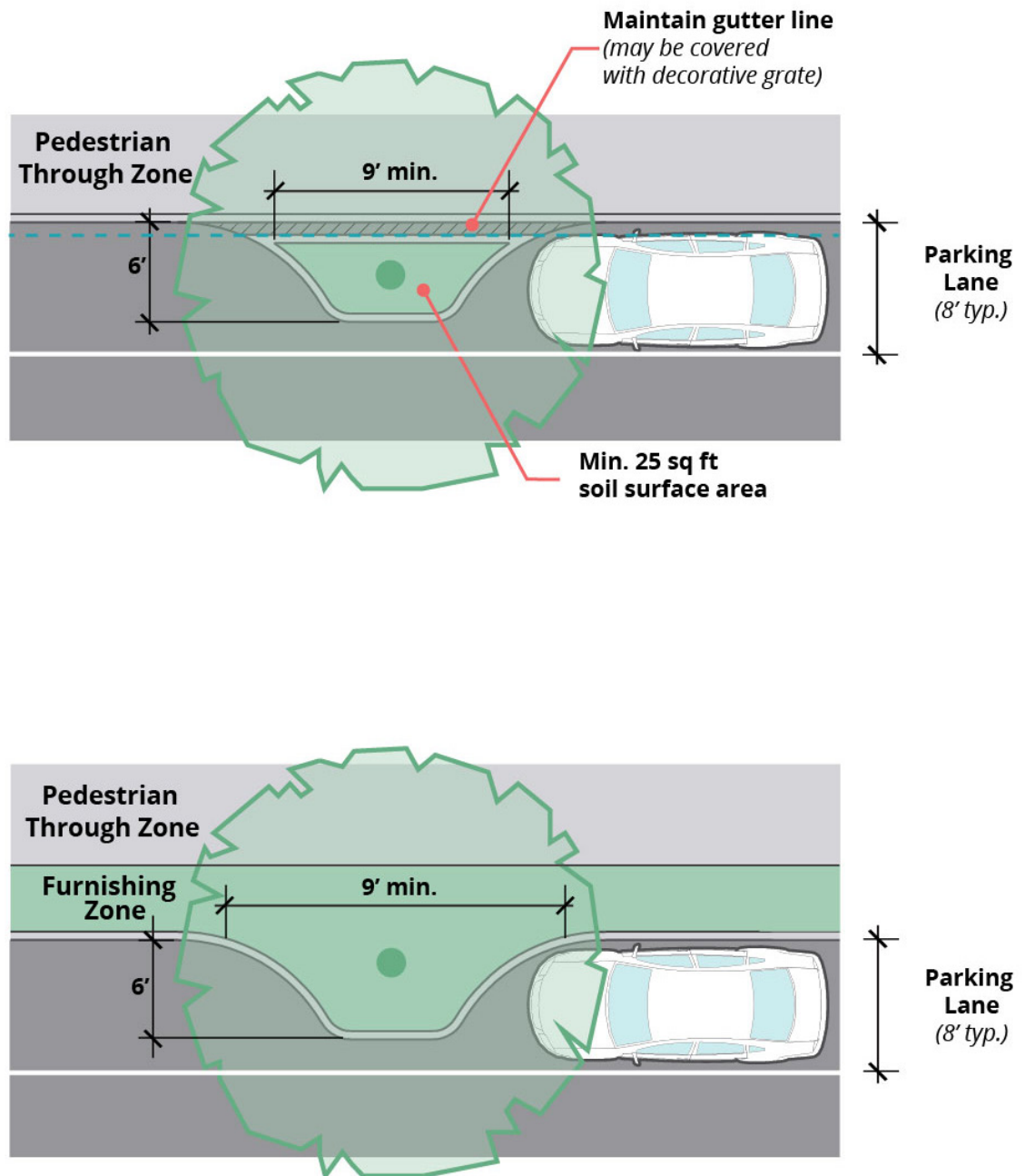
Figure B-28: Concepts for extending tree wells into the curb zone
