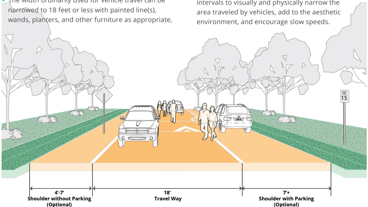
Figure B-36: Pedestrian Shared Street
