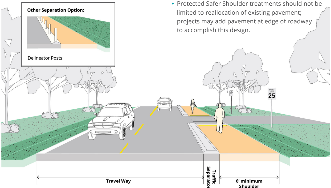
Figure B-40: Protected Safer Shoulder
