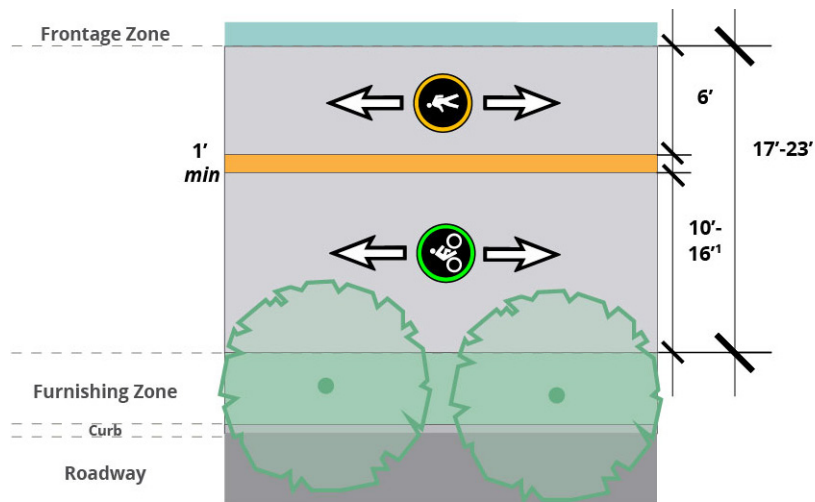
Figure B-21: Two-way Bicycle Multi-Use Path
