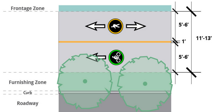
Figure B-19: Delineated Multi-Use Path (preferred)
