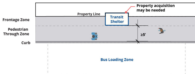
Figure B-13: Transit shelter siting on curb-tight sidewalks
