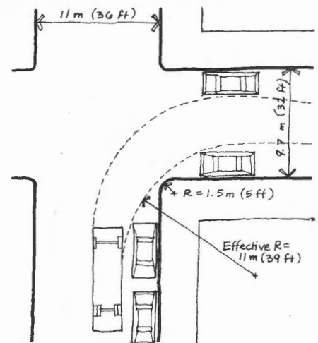
Where there is an effective curb radius sufficient for turning vehicles, the actual curb radius may be as small as 1.5 m. (5 ft).
