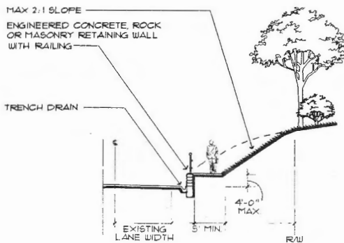
Separated Pathway on Wall
