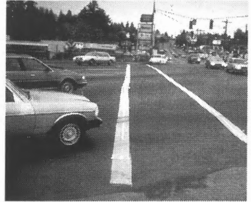
Very long crosswalks discourage pedestrian travel. Designers should avoid making crosswalks longer than 15 m (50'-0"). For wider streets, consider the use of median refuge islands.
