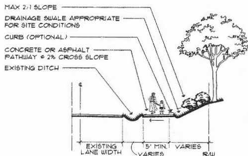
Separated Pathway with Swale
