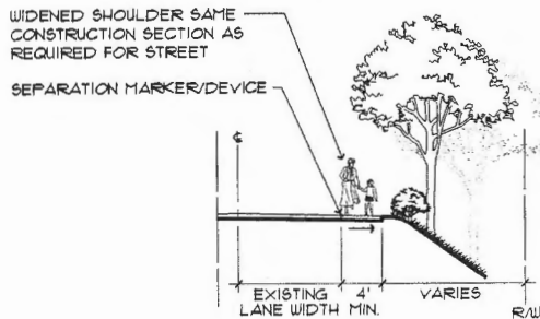
Widened Shoulder
