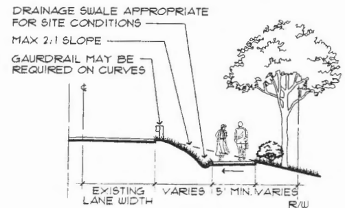
Separated Pathway below Road Grade
