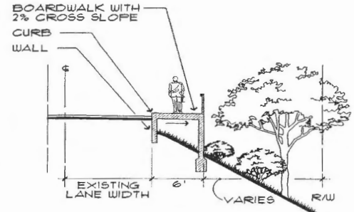
Separated Pathway on Boardwalk
