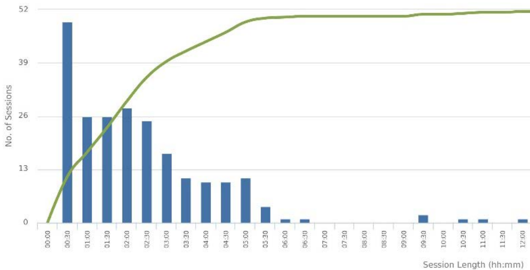
Figure 18. Charging Session Length at Select Customer Owned Level 2 Chargers
