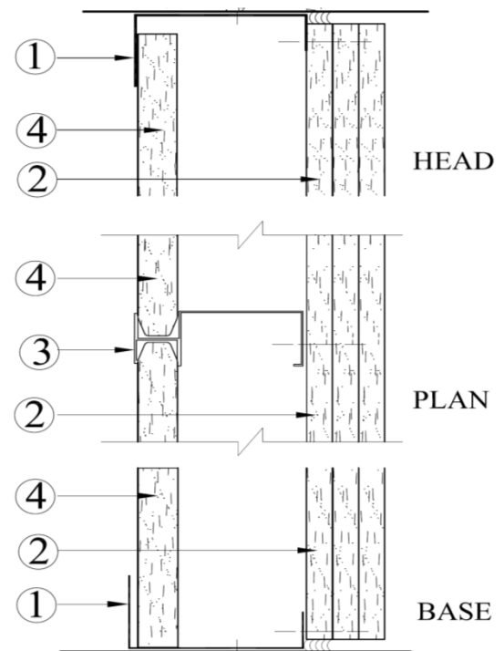
Figure 4 - 3-HR Cavity Shaft Wall (Non-Load Bearing)
