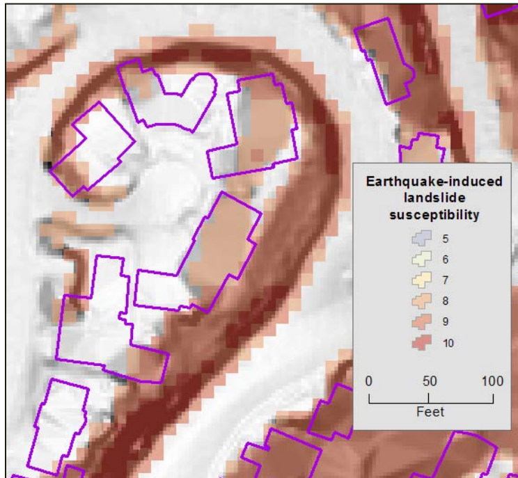
Figure 3-1. Example: Capturing the variability of landslide susceptibility within building footprints (magenta polygons). Landslide susceptibility values use the Hazus landslide susceptibility 0 through 10 scale. Areas of no shading: minimal to no landslide susceptibility. Earthquake-induced landslide susceptibility data from Appleby and others (in preparation).
