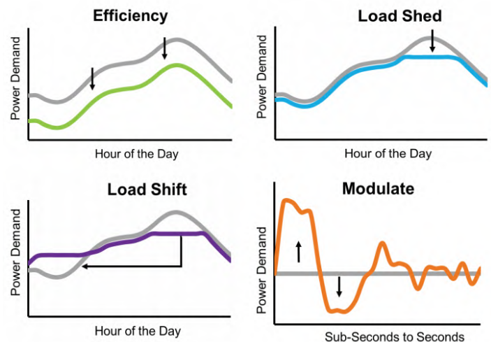
Figure 4. Building load strategies and flexibility modes 1
