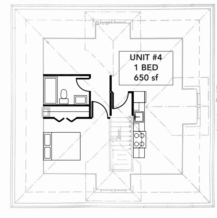
PLAN Attic 650 sf
