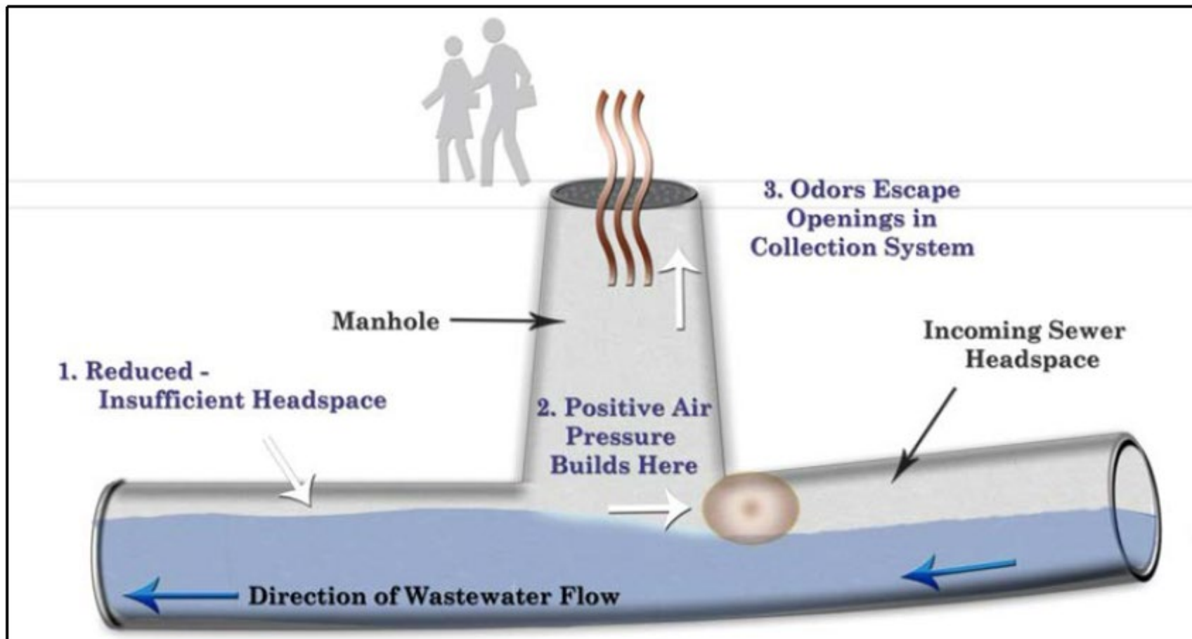
Figure 4. Headspace airflow restriction in a gravity sewer pipe
