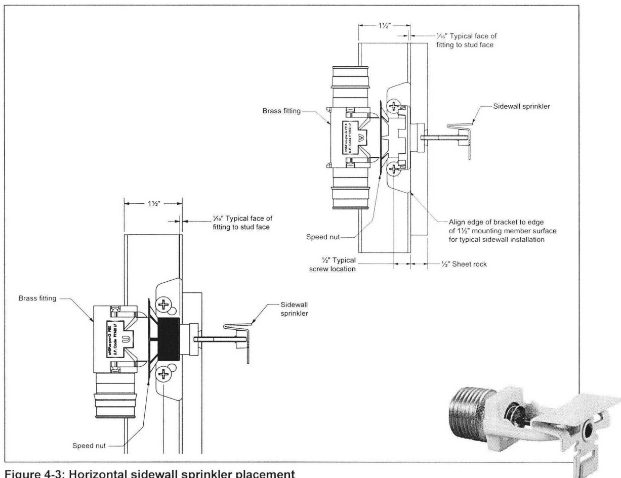
Figure 4-3: Horizontal sidewall sprinkler placement
