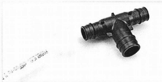
Figure 1-4: Uponor PEX tubing, ProPEX ring and ProPEX EP tee
