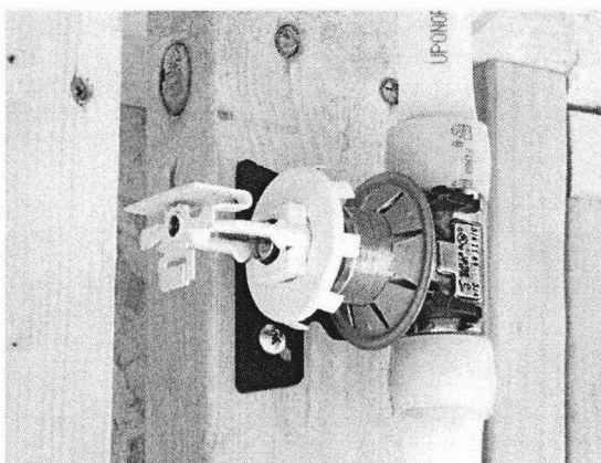
Figure 1-3: ProPEX tee with horizontal sidewall sprinkler
