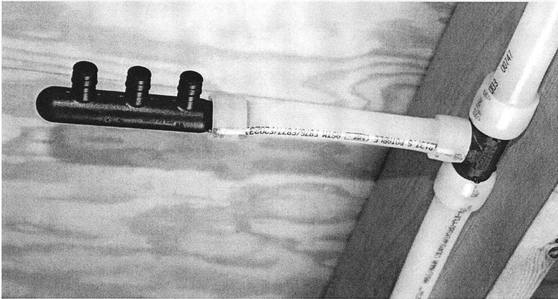
Figure 7-1: Feed plumbing fixtures via EP multiport tees
