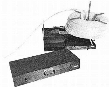
Figure 6-25: Compact select uncoiler (E6063000)
