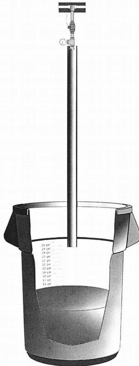
Figure 10-3: Flow test bucket
