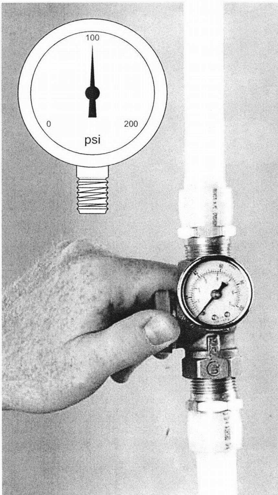
Figure 9-1: Pressure test at normal operating water pressure
