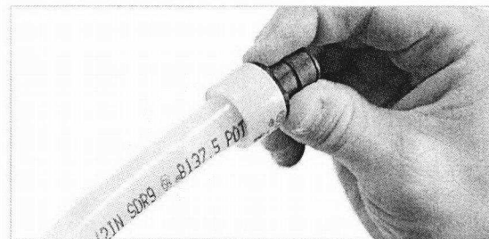
Figure 6-12: Insert fitting
