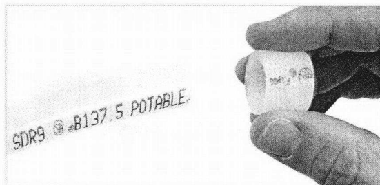
Figure 6-10: Install ProPEX ring
