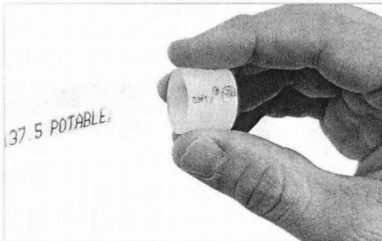
Figure 6-2: Install ProPEX ring
