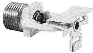
Figure 1-9: Recessed horizontal sidewall sprinkler
