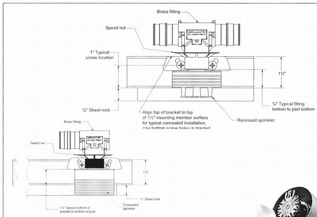
Figure 4-2: Concealed assembly sprinkler placement
