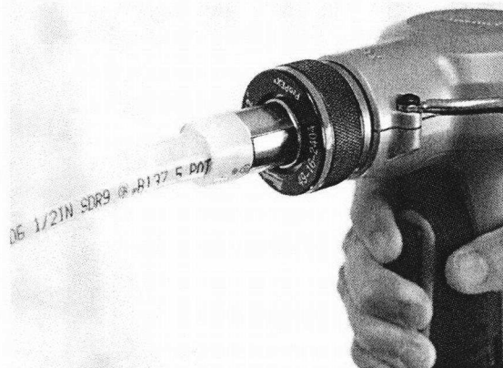
Figure 6-4: Expand until ring is snug against expander head
