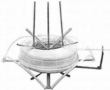
Figure 6-22: Tube uncoiler (E6061000)
