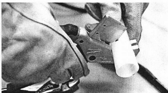
Figure 6-17: Cut tubing
