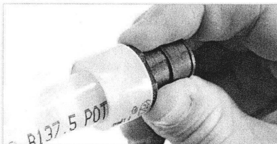
Figure 6-8: Ensure tubing and ring seat against shoulder of fitting
