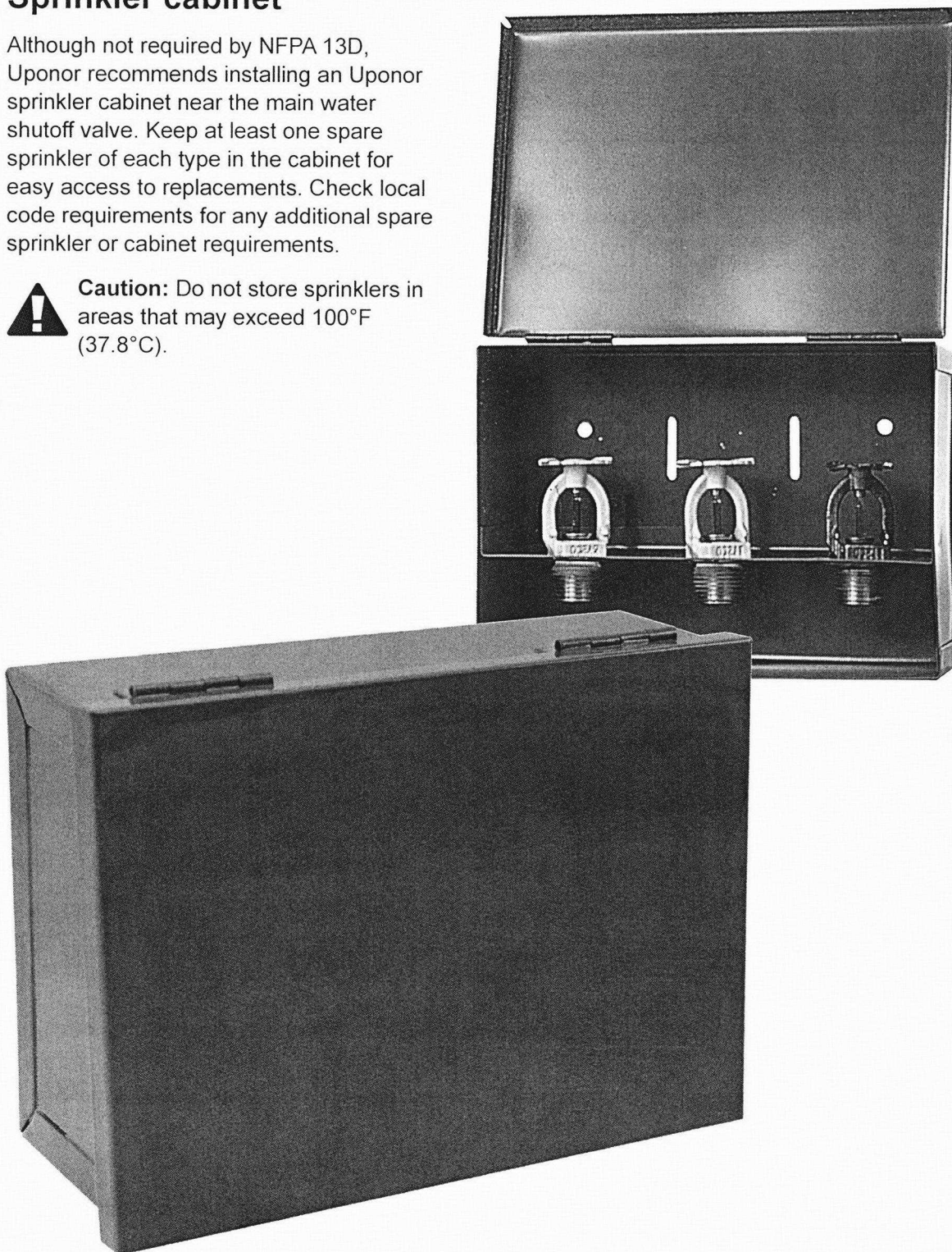
Figure 11-1: Sprinkler cabinet
