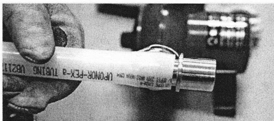
Figure 6-14: Gently heat tubing
