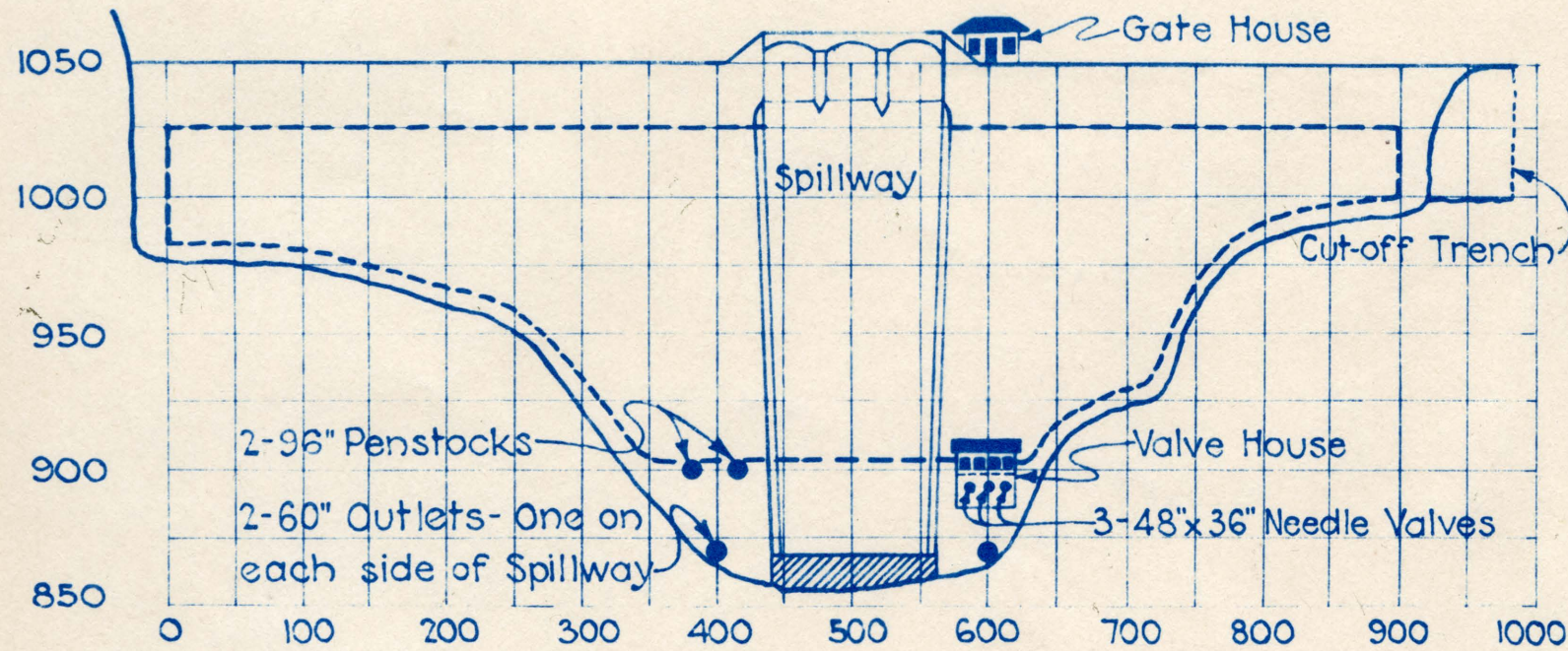
BULL RUN DAM DOWNSTREAM ELEVATION
