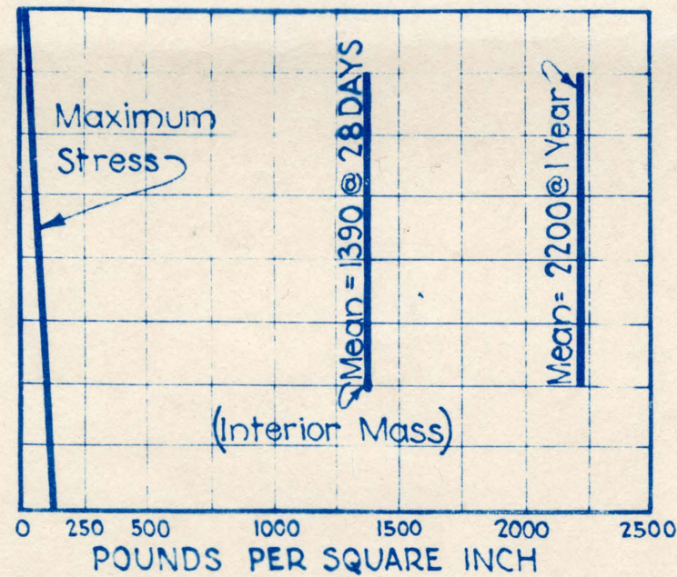
STRESS-STRENGTH RELATION INTERIOR MASS CONCRETE
