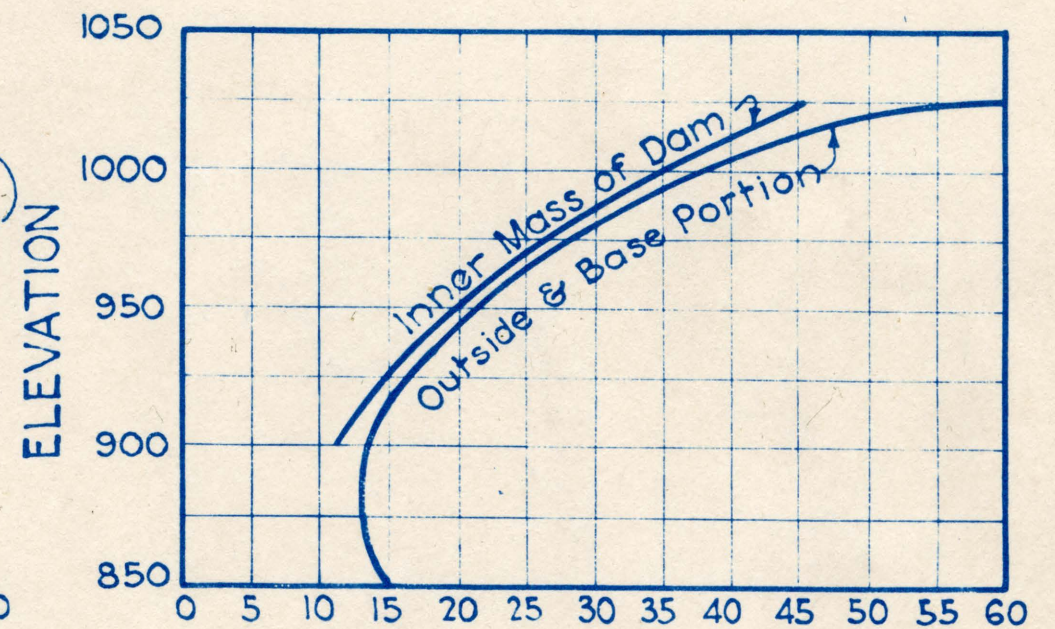
RATIO: \frac{\text{1 YEAR STRENGTH}}{\text{STRESS}}
