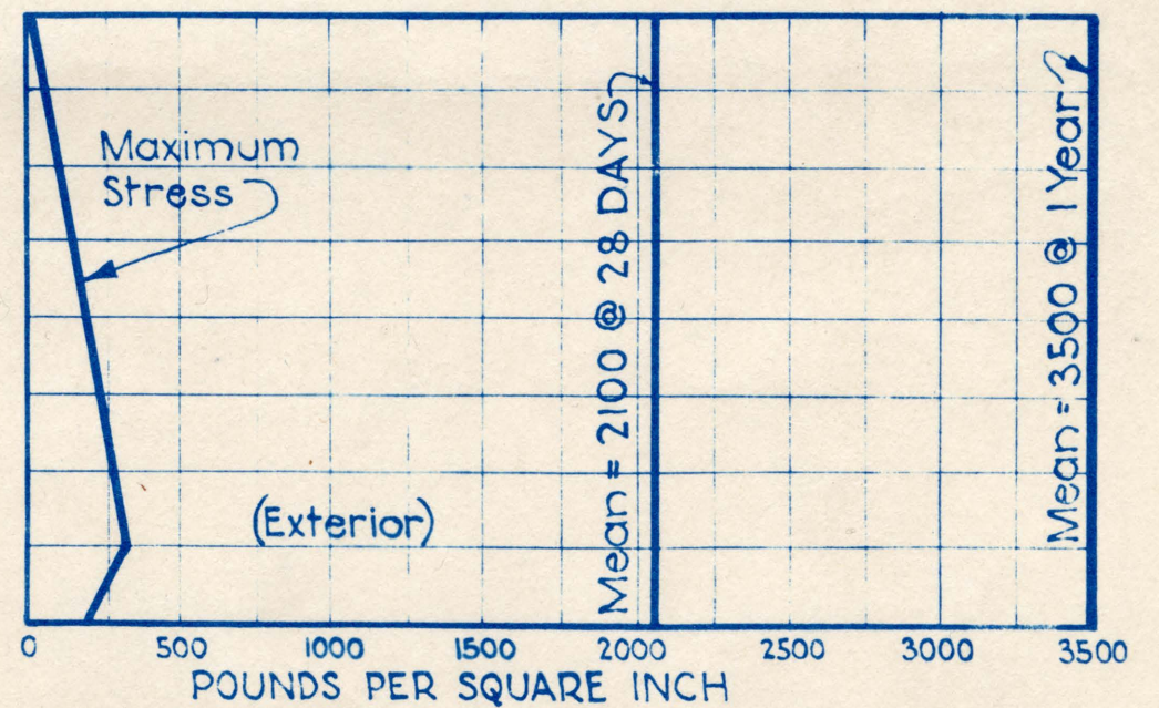
STRESS-STRENGTH RELATION FOUNDATION & EXTERIOR CONCRETE
