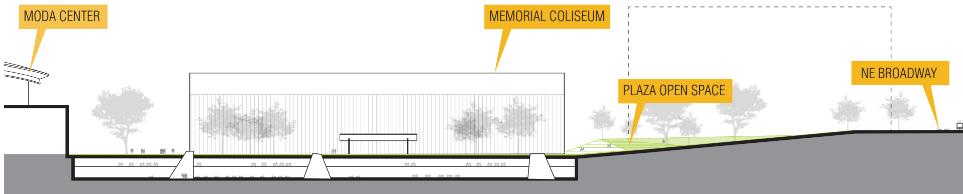
PUBLIC PLAZA SECTION
