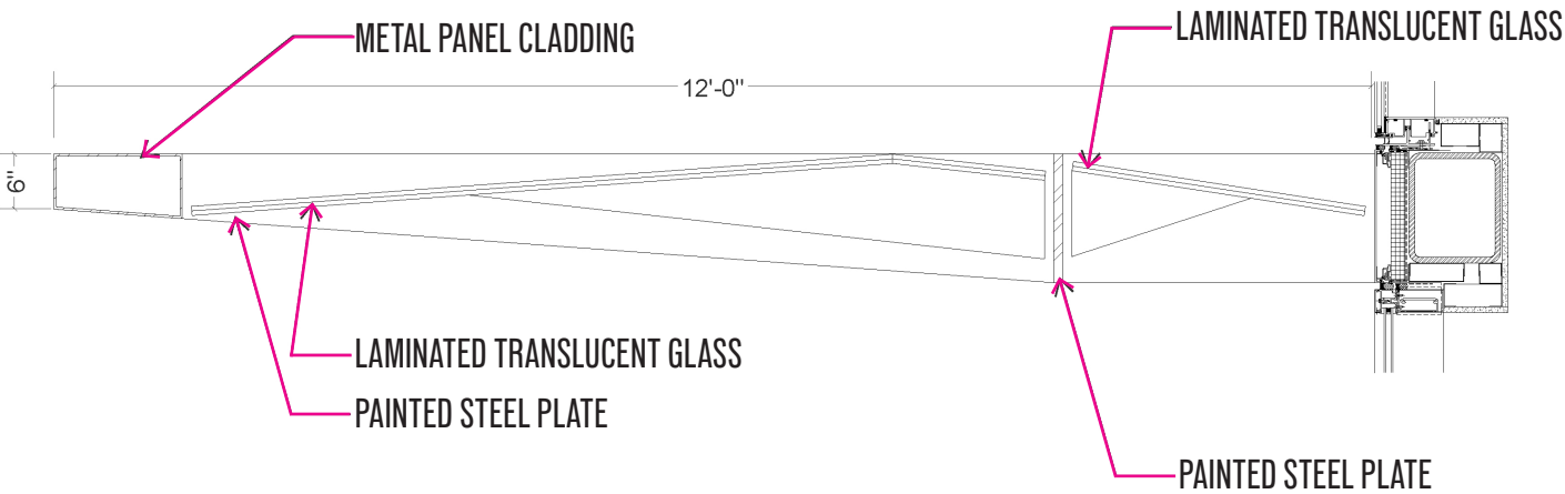
TYPE 2 - STEEL AND GLASS
