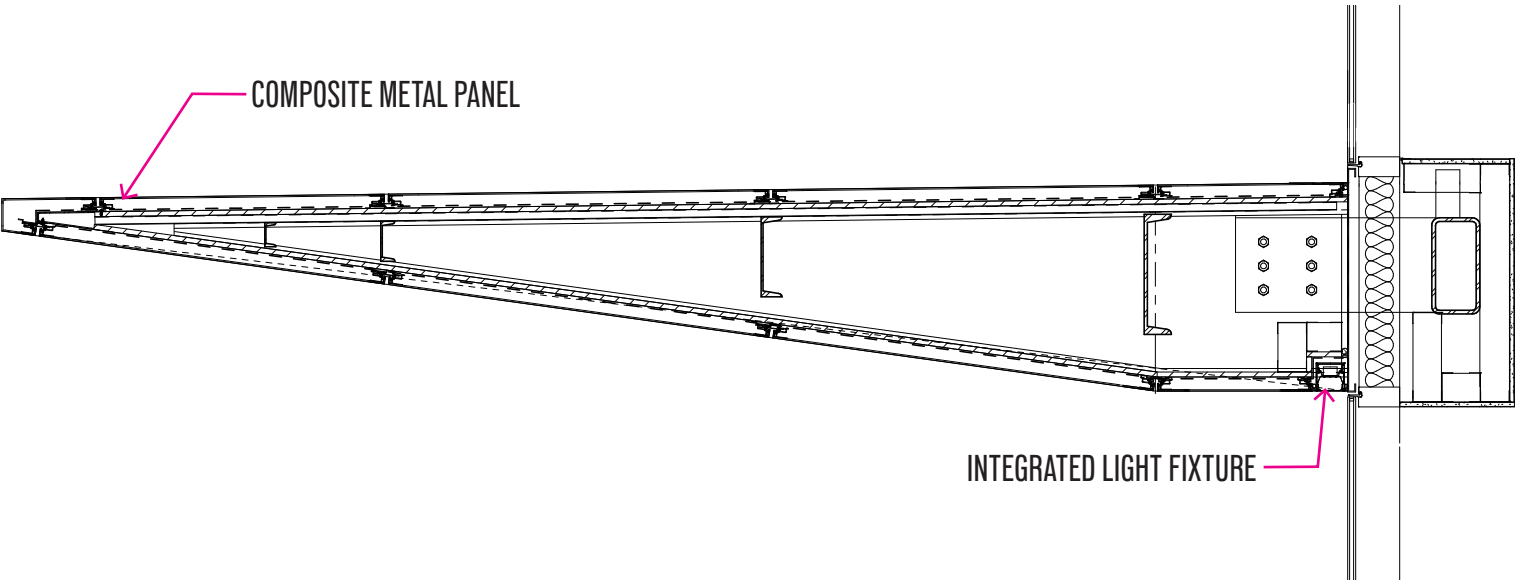
TYPE 3 - FACETED COMPOSITE METAL PANEL
