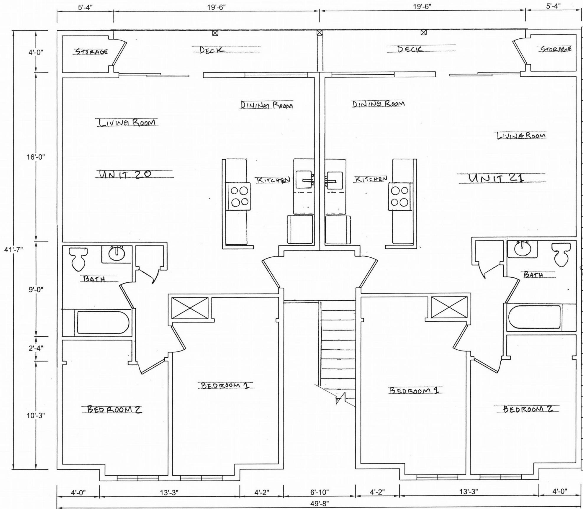
UPPER LEVEL FLOOR PLAN \frac{3}{16}'' = 1'-0''
