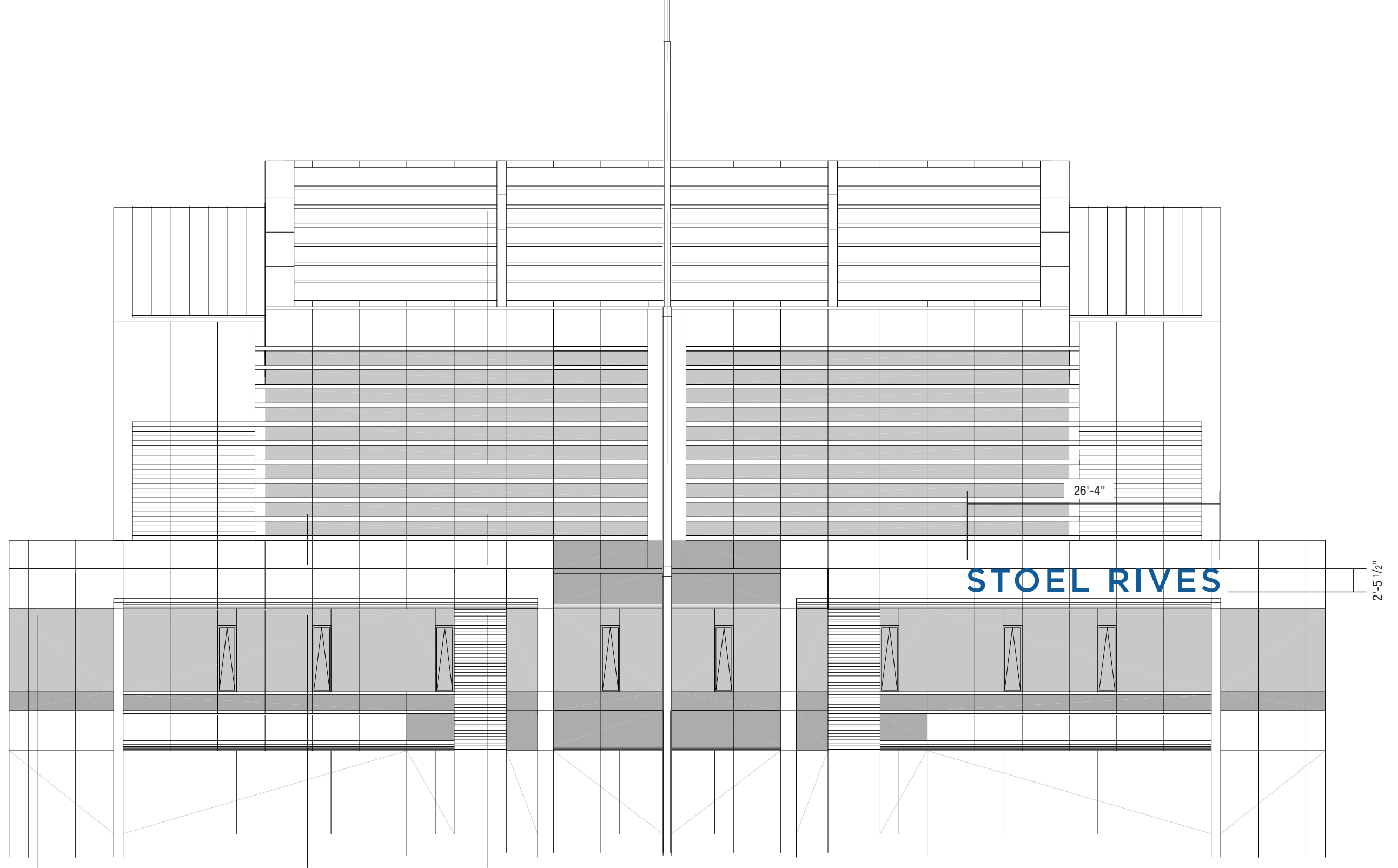
1 | EAST ELEVATION / PARAPET SIGN 3/32" = 1'-0" 64.7 SQFT.
