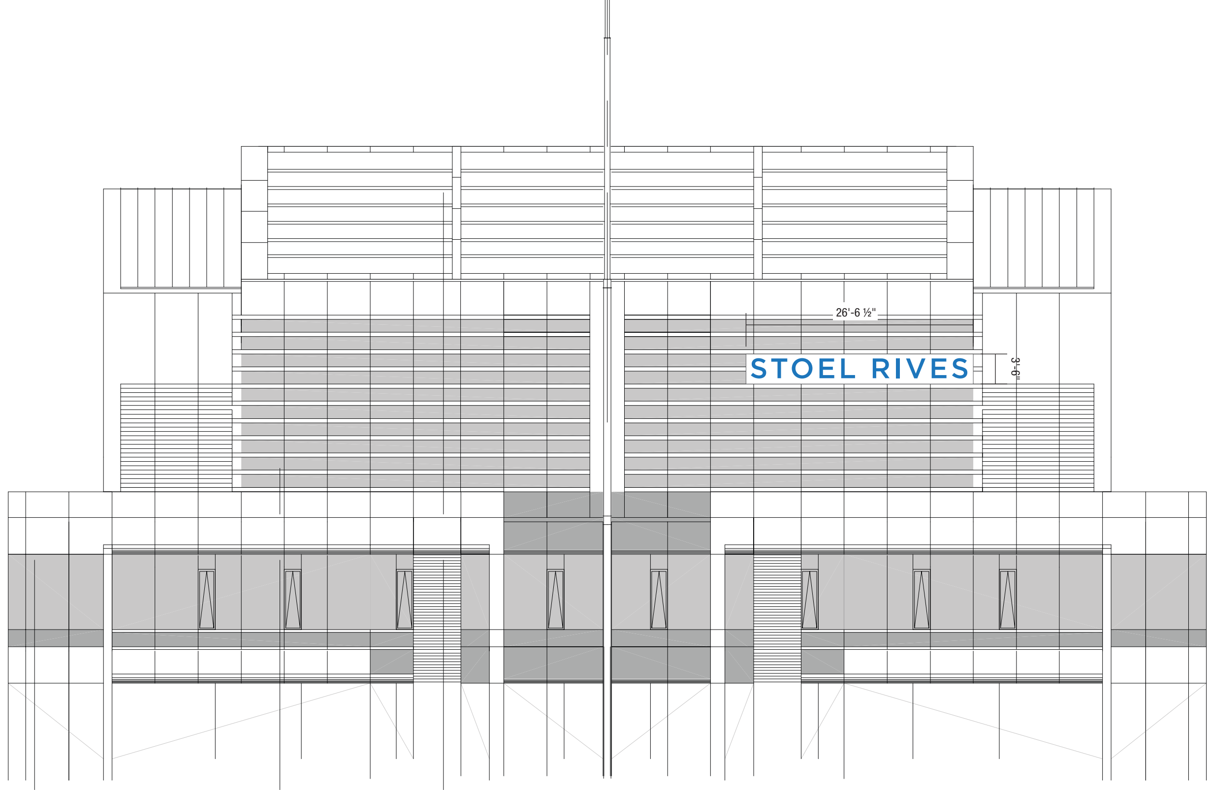
1 | EAST ELEVATION / LANTERN SIGN 3/32" = 1'-0" 56.1 SQFT. TEXT AREA / 92.75 SQFT. PANEL BACKER
