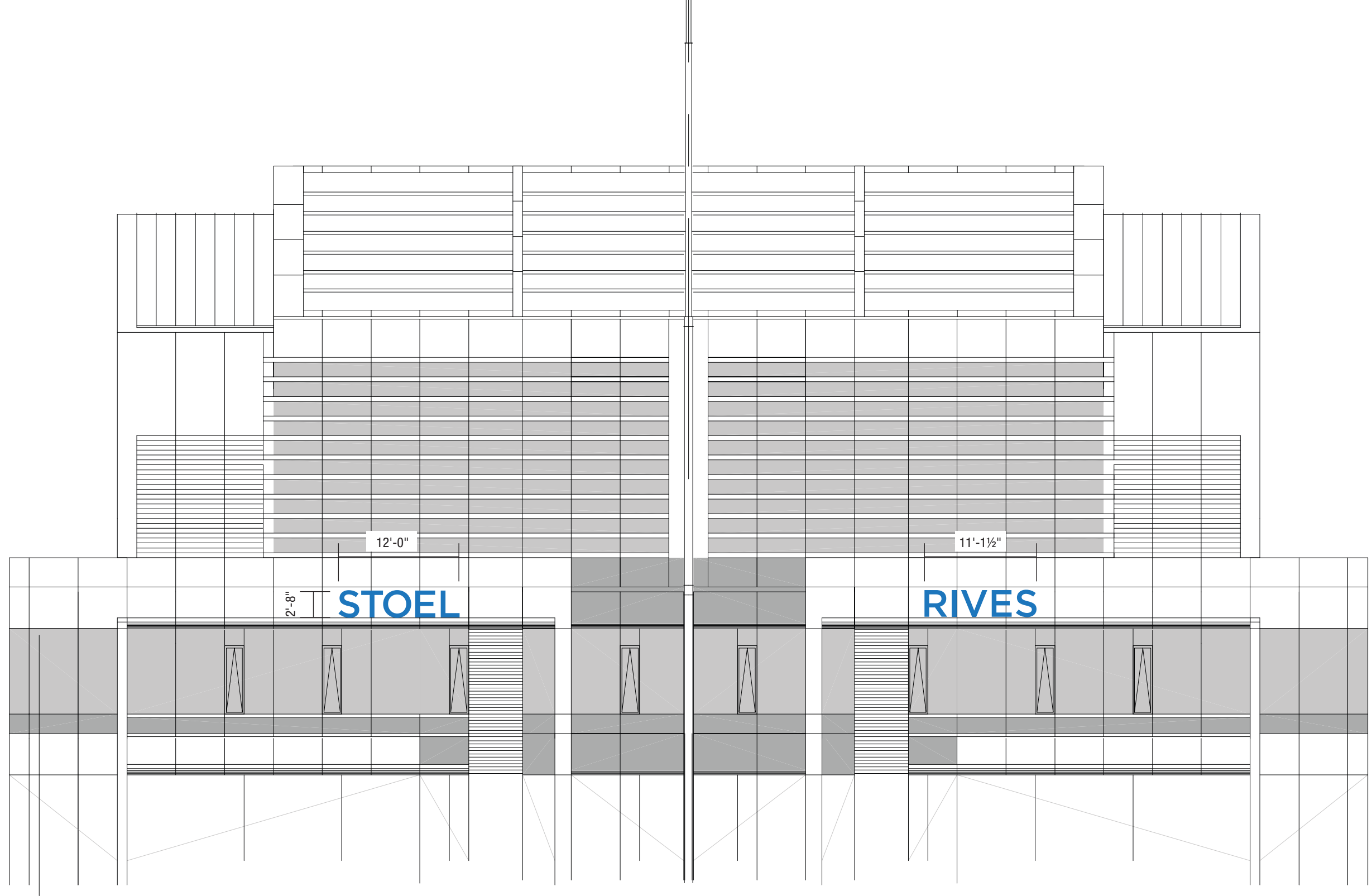
1 | EAST ELEVATION / PARAPET SIGN 3/32" = 1'-0" 32 SQFT. EACH
