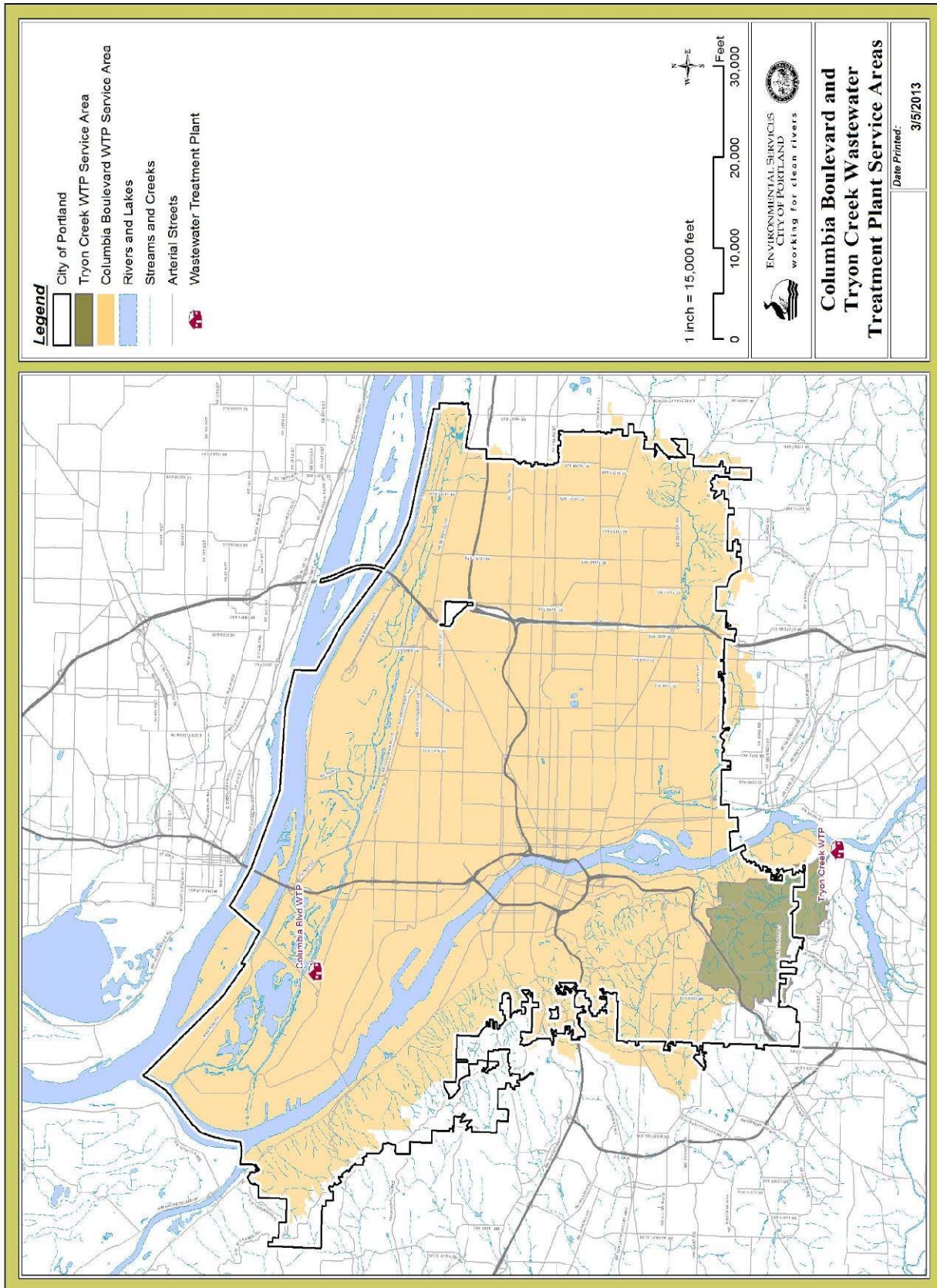
Figure 6.9 Columbia Boulevard and Trvon Creek Wastewater Treatment Plants Service Areas
