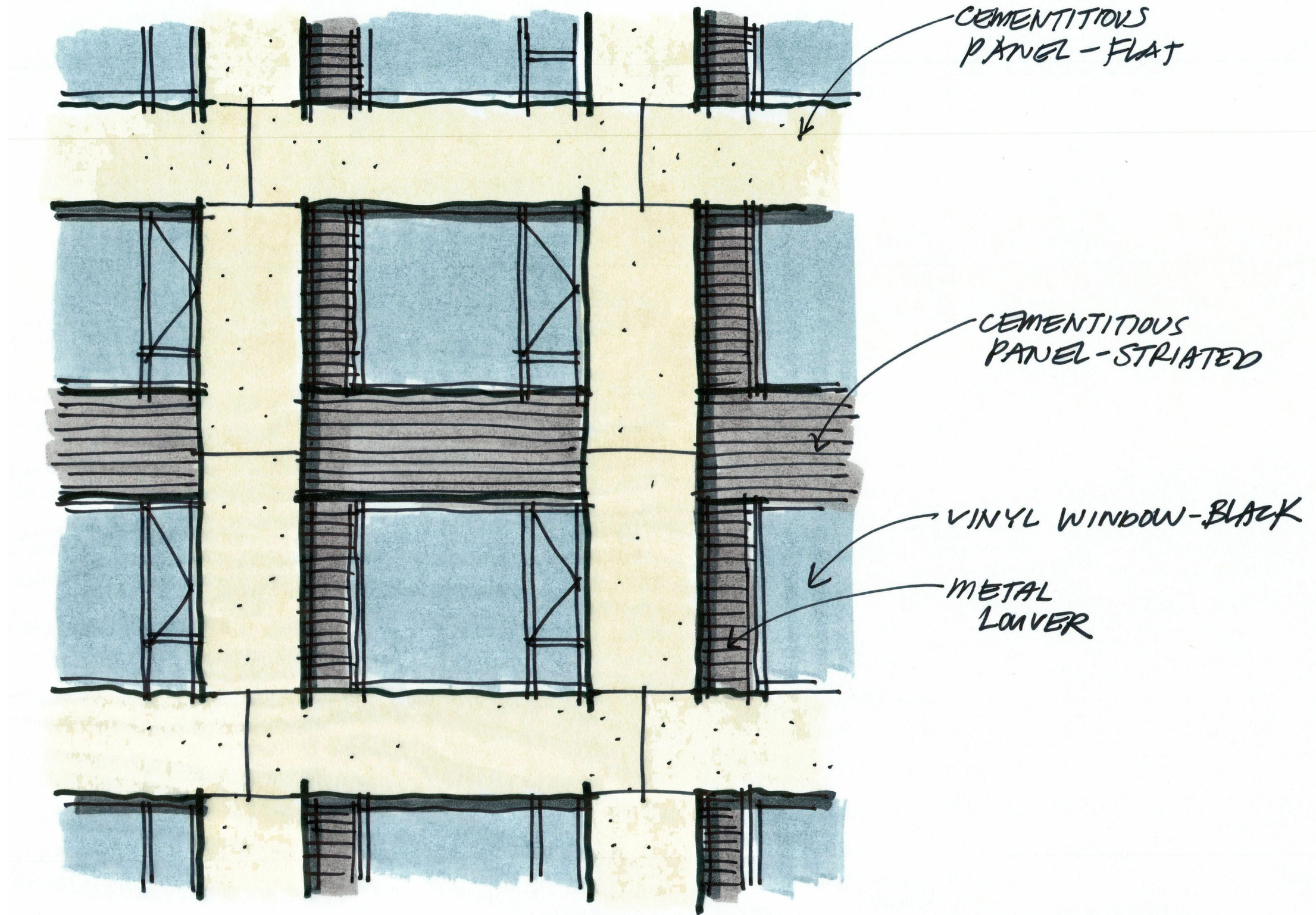
TYPICAL WALL
