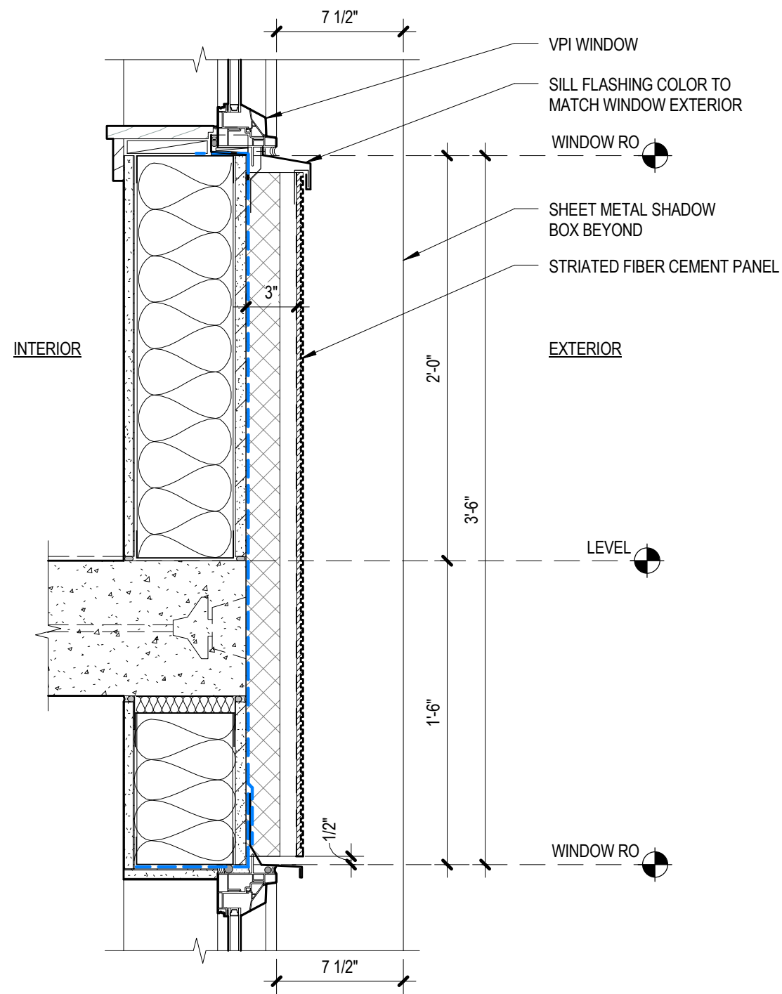
2 WINDOW HEAD/SILL @ SHALLOW WALL
