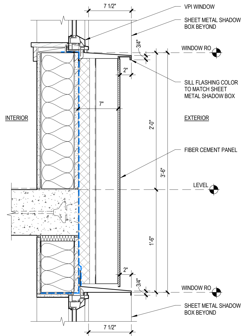
1 WINDOW HEAD/SILL @ DEEP WALL
